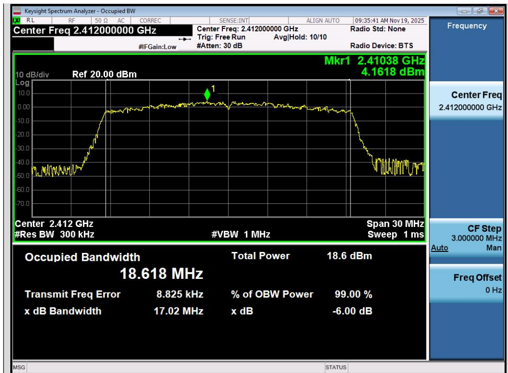
Test_Graph_802.11ax20_Chain A_2412_MCS0_DTSBW
