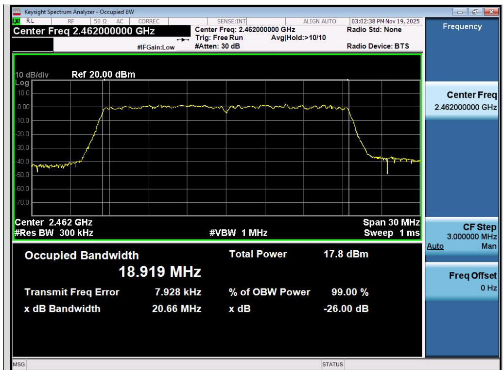
Test_Graph_802.11ax20_Chain B_2462_MCS0_OBW
