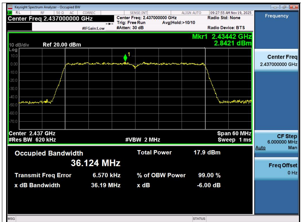
Test_Graph_802.11n40_Chain A_2437_MCS0_DTSBW
