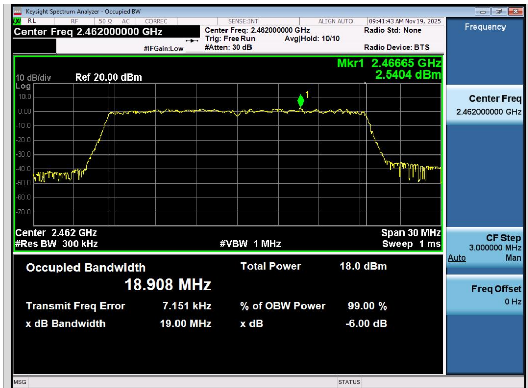
Test_Graph_802.11ax20_Chain A_2462_MCS0_DTSBW
