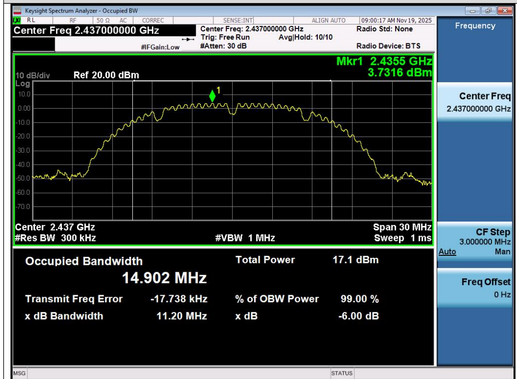
Test_Graph_802.11b_Chain A_2437_1Mbps_DTSBW
