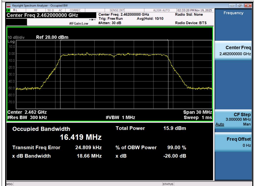
Test_Graph_802.11g_Chain B_2462_6Mbps_OBW
