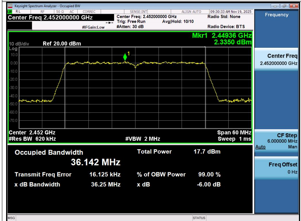
Test_Graph_802.11n40_Chain A_2452_MCS0_DTSBW
