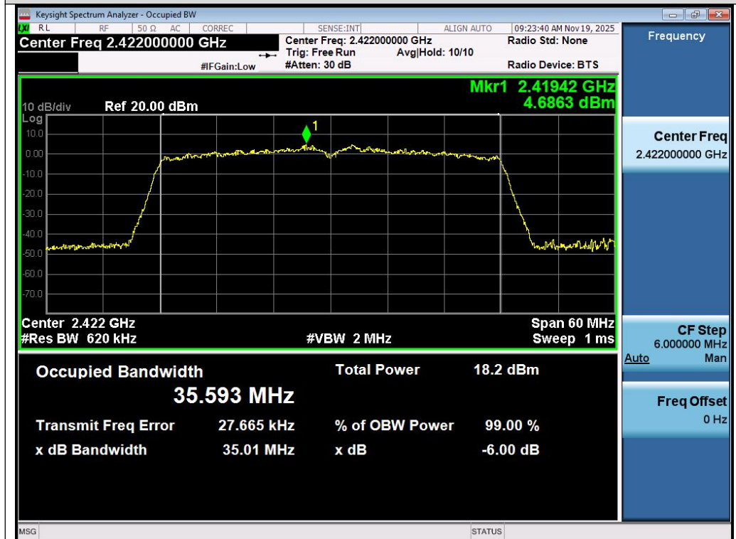
Test_Graph_802.11n40_Chain A_2422_MCS0_DTSBW
