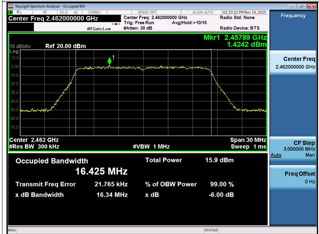
Test_Graph_802.11g_Chain B_2462_6Mbps_DTSBW
