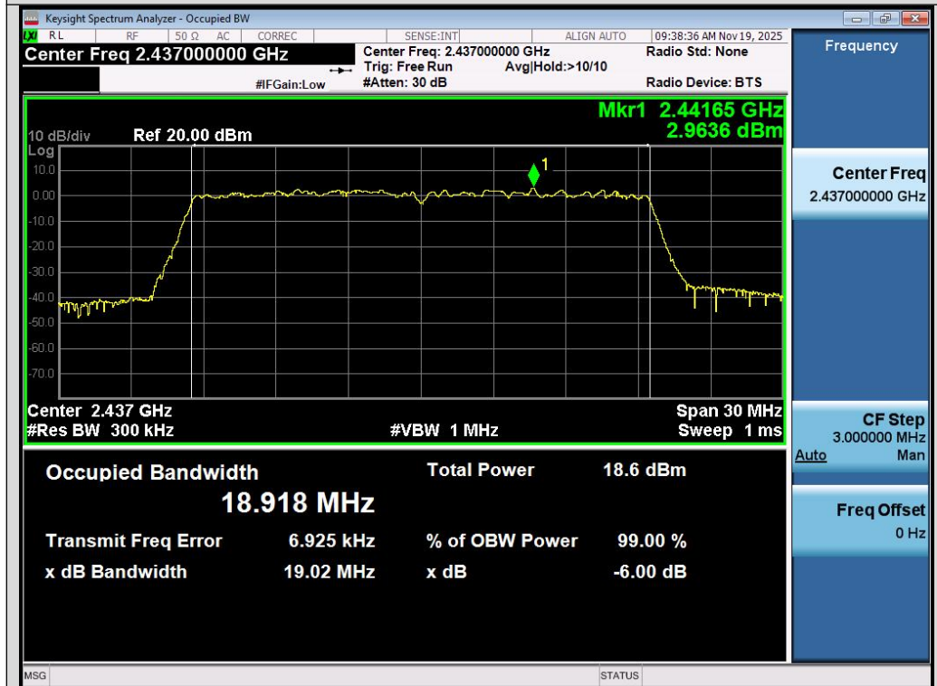
Test_Graph_802.11ax20_Chain A_2437_MCS0_DTSBW
