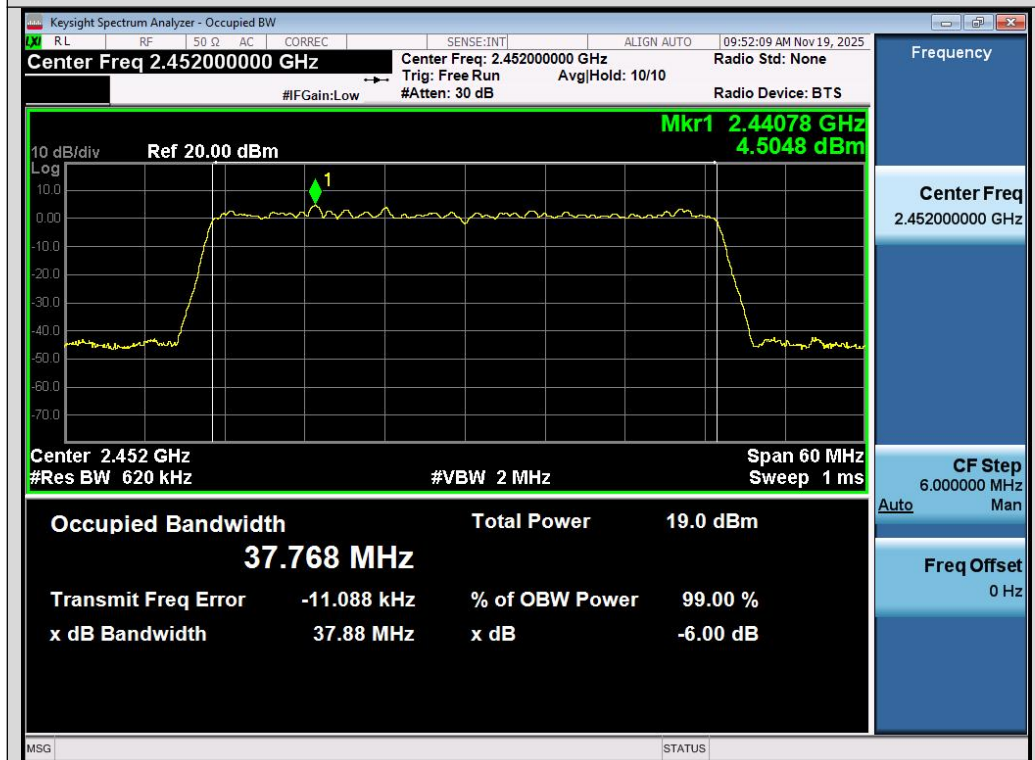
Test_Graph_802.11ax40_Chain A_2452_MCS0_DTSBW
