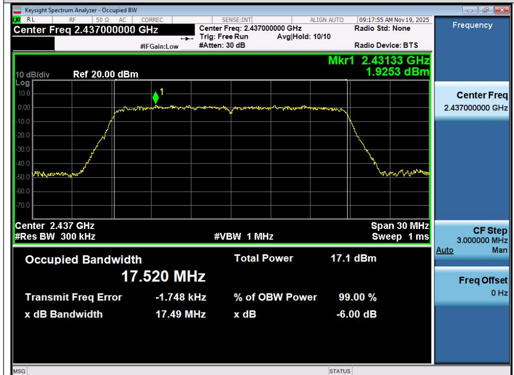
Test_Graph_802.11n20_Chain A_2437_MCS0_DTSBW
