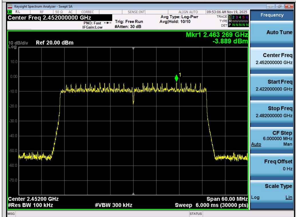
Test_Graph_802.11ax40_Chain A_2452_MCS0_Reference Level
