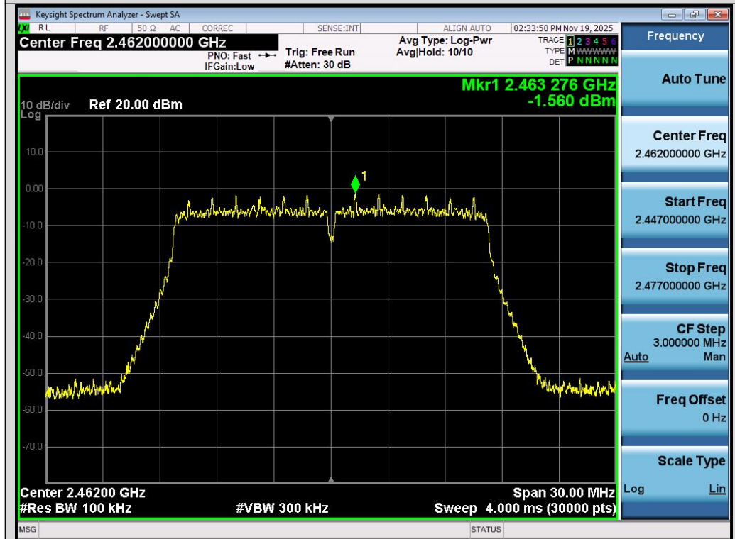
Test_Graph_802.11g_Chain B_2462_6Mbps_Reference Level
