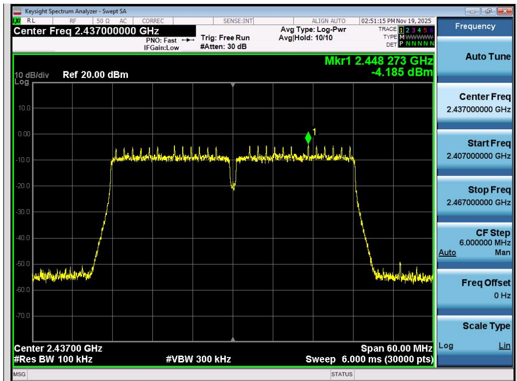
Test_Graph_802.11n40_Chain B_2437_MCS0_Reference Level
