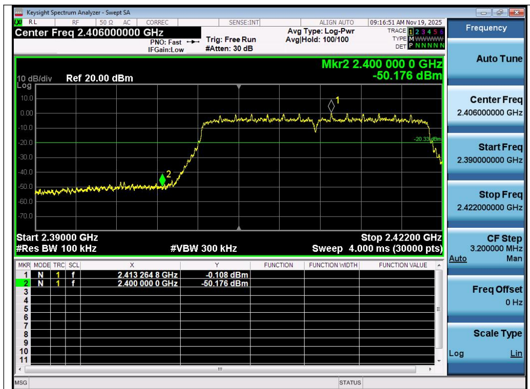
Test_Graph_802.11n20_Chain A_2412_MCS0_Lower Band Edge Emissions
