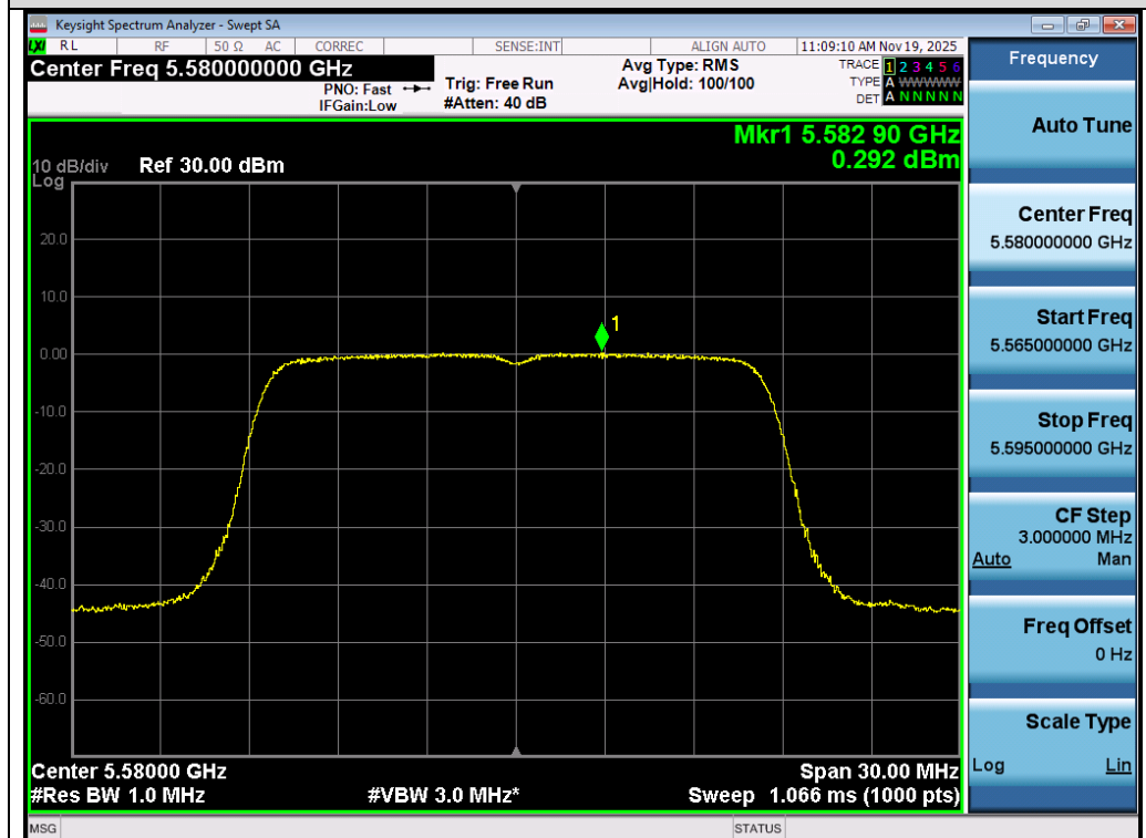
Test_Graph_802.11a_Chain A_5580_6Mbps_PSD
