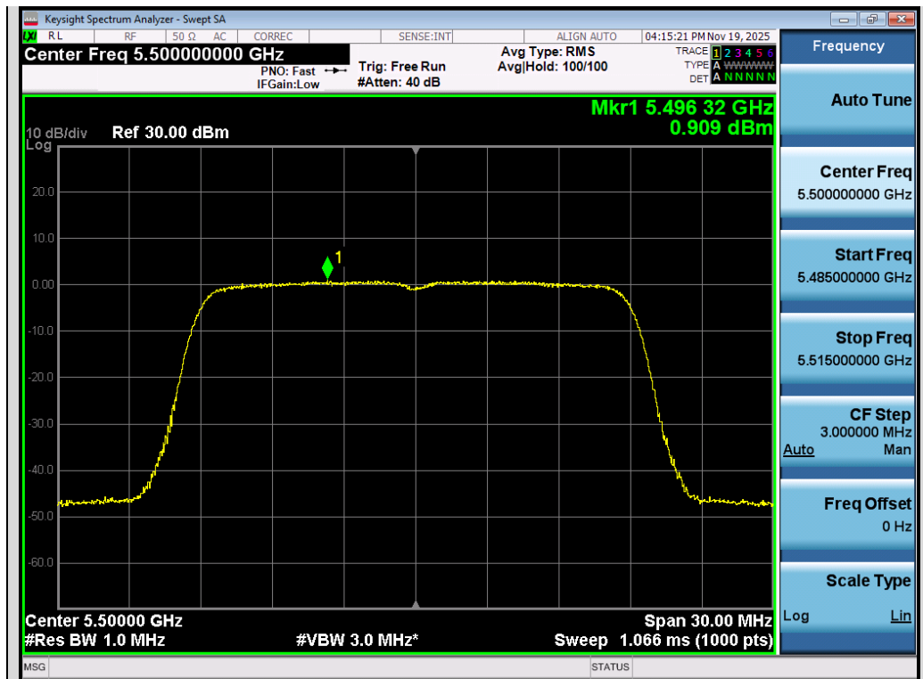
Test_Graph_802.11n20_Chain B_5500_MCS0_PSD
