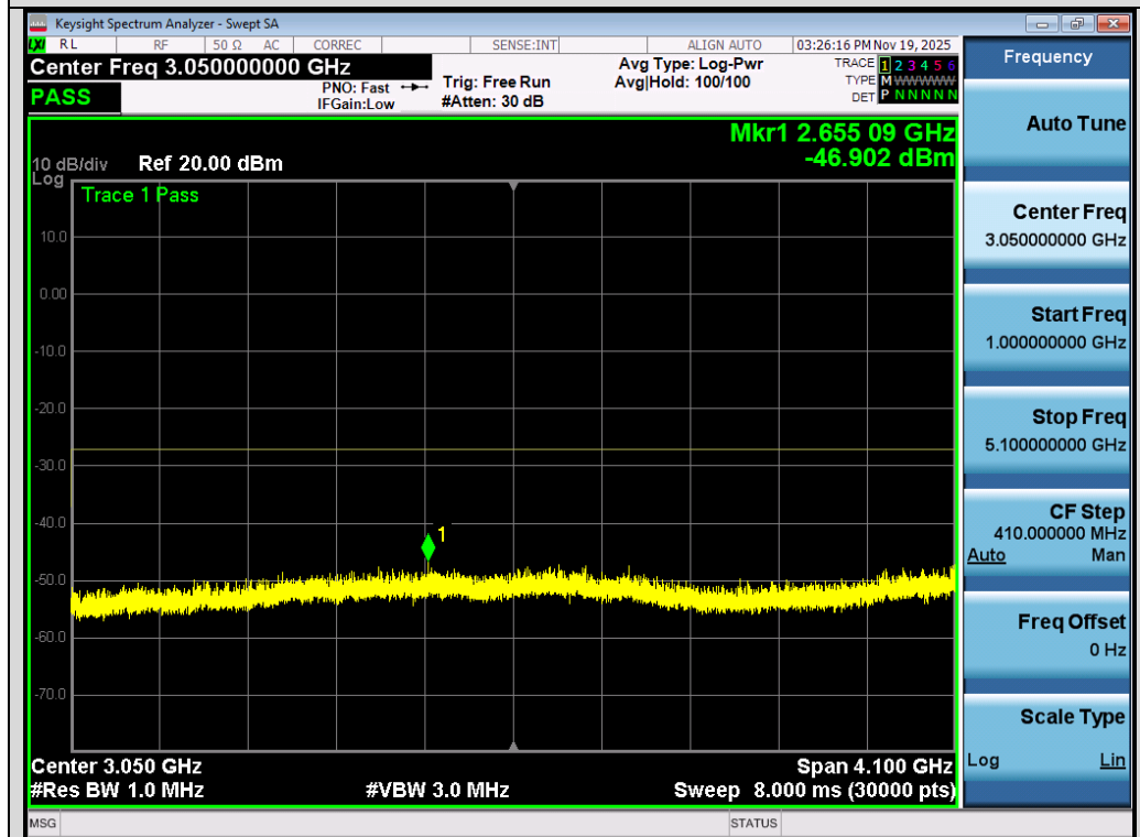
Test_Graph_802.11n40_Chain B_5190_MCS0_Frequency Band 2
