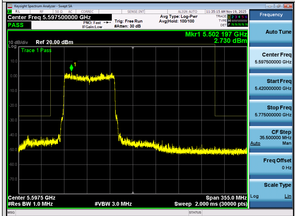
Test_Graph_802.11ax80_Chain A_5530_MCS0_Frequency Band 3
