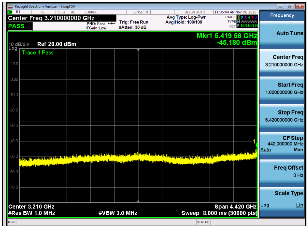
Test_Graph_802.11ax80_Chain A_5530_MCS0_Frequency Band 2
