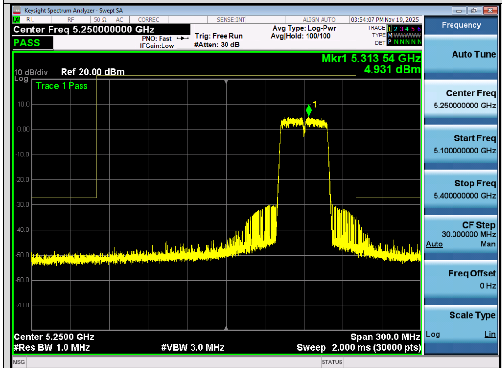
Test_Graph_802.11n40_Chain B_5310_MCS0_Frequency Band 3
