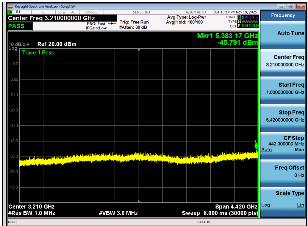
Test_Graph_802.11a_Chain B_5500_6Mbps_Frequency Band 2
