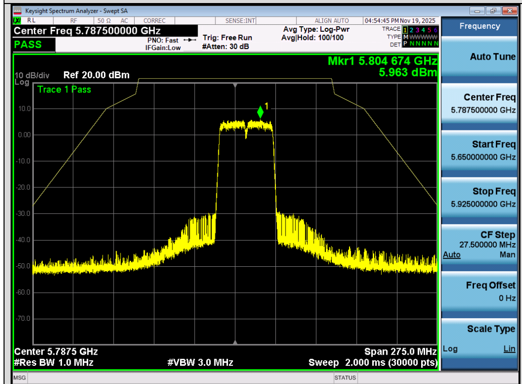
Test_Graph_802.11n40_Chain B_5795_MCS0_Frequency Band3
