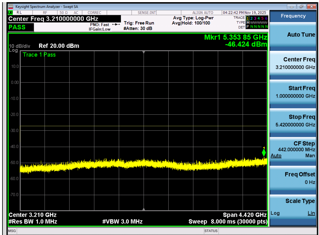
Test_Graph_802.11n40_Chain B_5670_MCS0_Frequency Band 2
