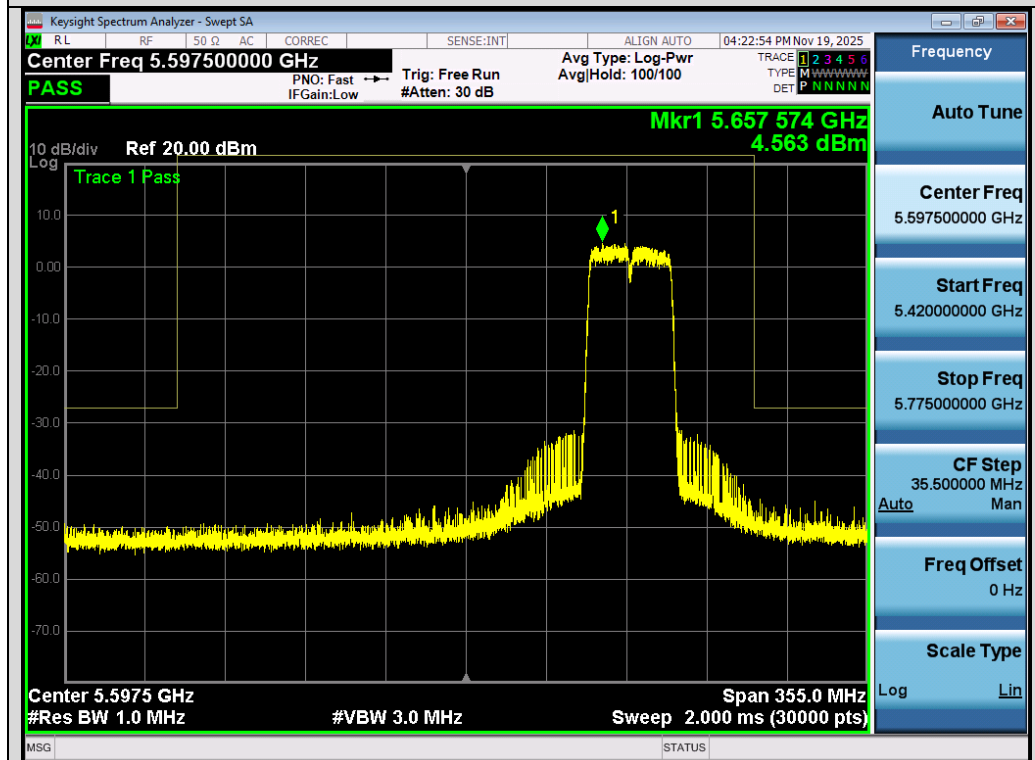
Test_Graph_802.11n40_Chain B_5670_MCS0_Frequency Band 3
