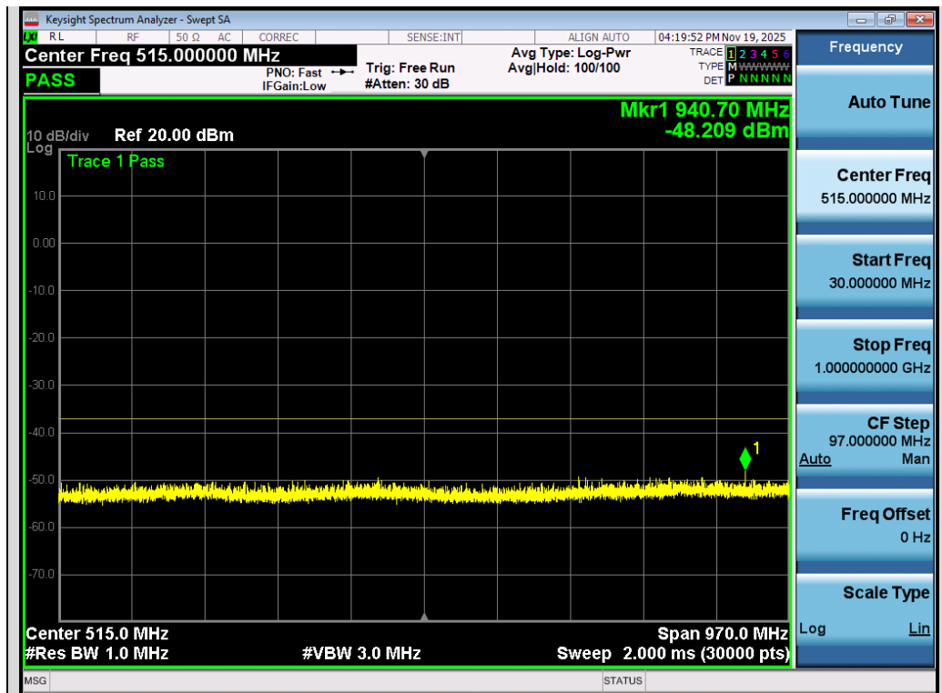
Test_Graph_802.11n40_Chain B_5550_MCS0_Frequency Band 1
