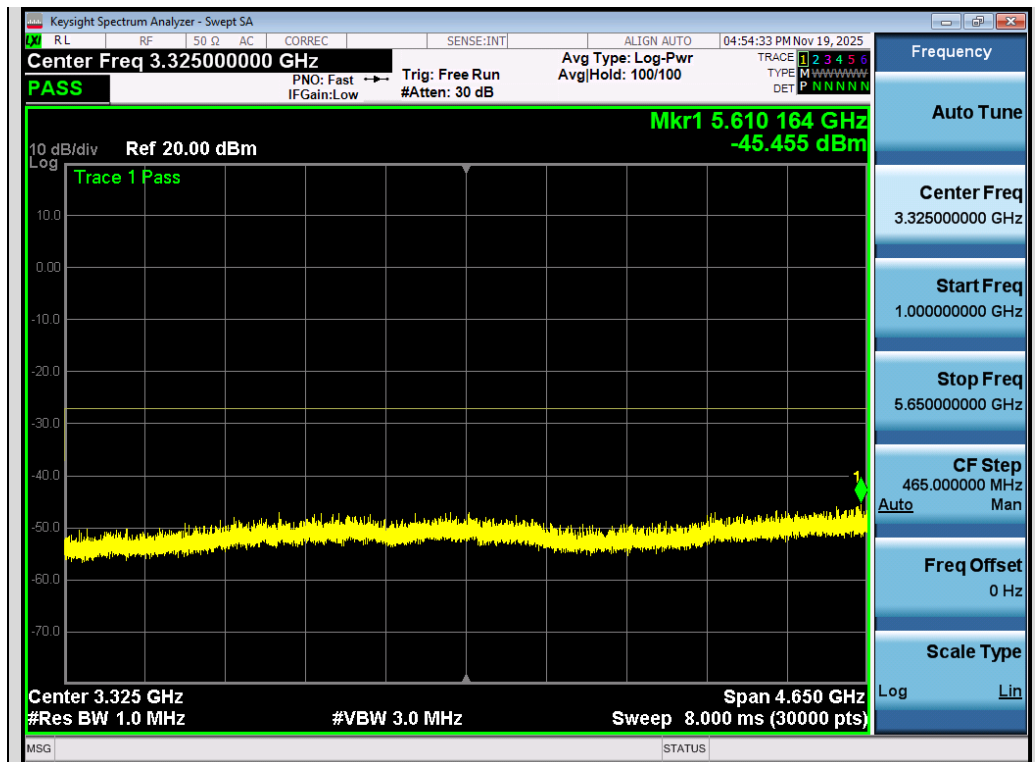
Test_Graph_802.11n40_Chain B_5795_MCS0_Frequency Band2
