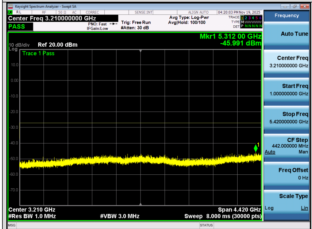
Test_Graph_802.11n40_Chain B_5550_MCS0_Frequency Band 2
