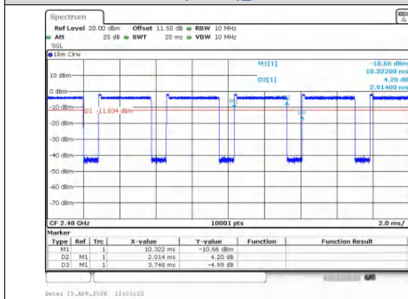
8DPSK(3-DH5)_Channel 78
