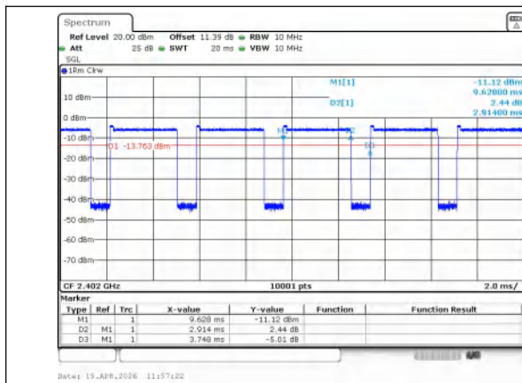
8DPSK(3-DH5)_Channel 0
