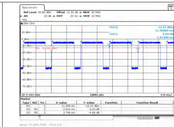
8DPSK(3-DH5)_Channel 39
