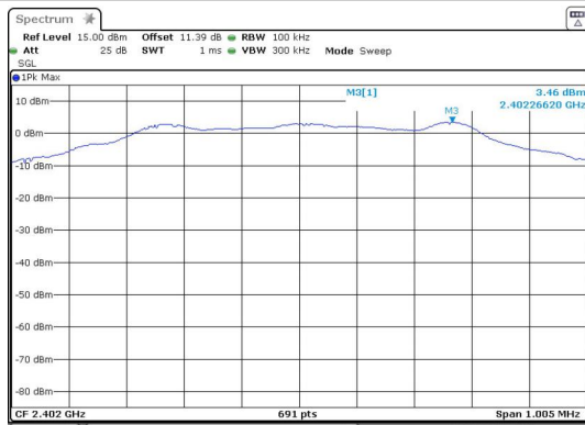
In-Band Reference Level BLE 1M_Channel 0
