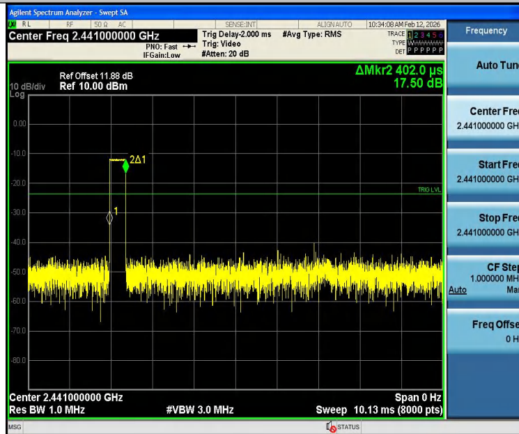
2DH1-Ant1-Hop-PASS
