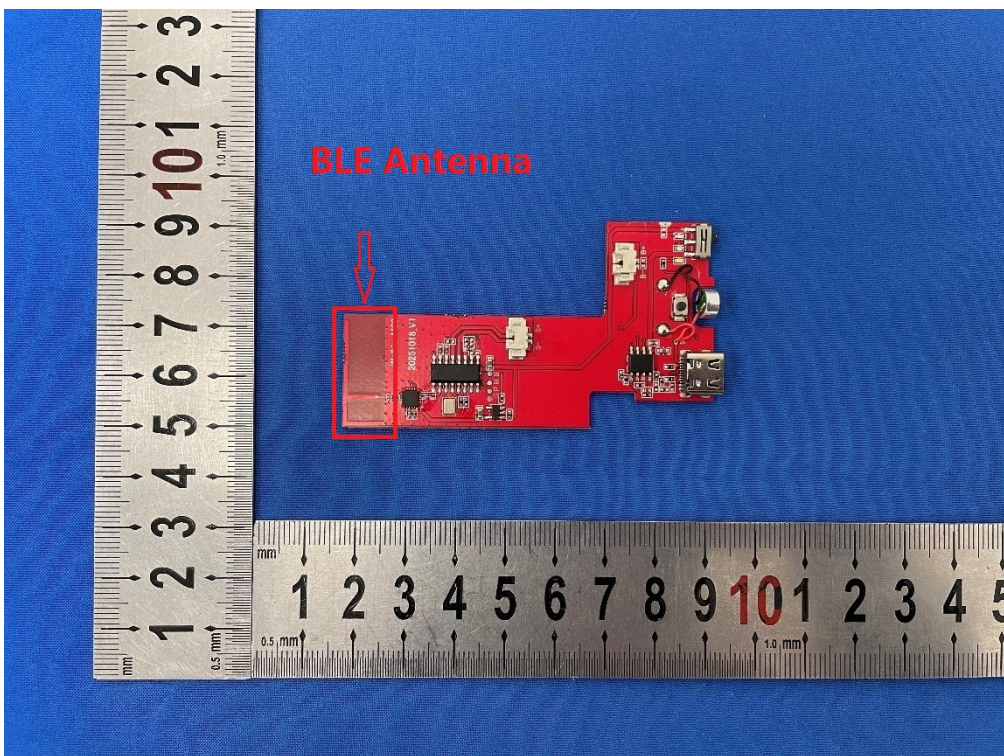
Photo 4: Internal View for BLE Antenna
