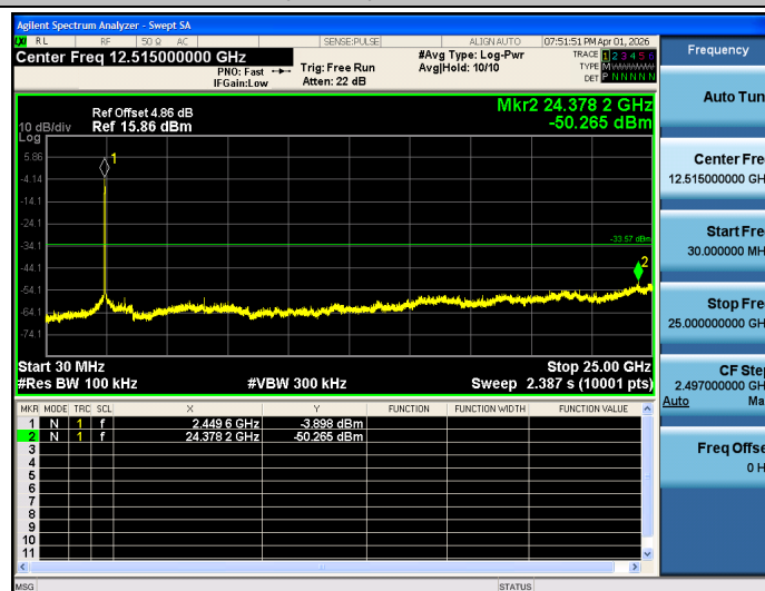
802.11n(HT40)_2452_30~25000
