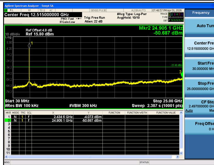
802.11n(HT40)_2452_0~Reference
