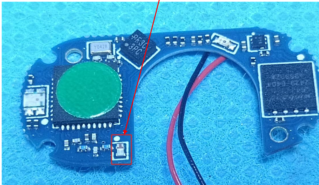
RF antenna
