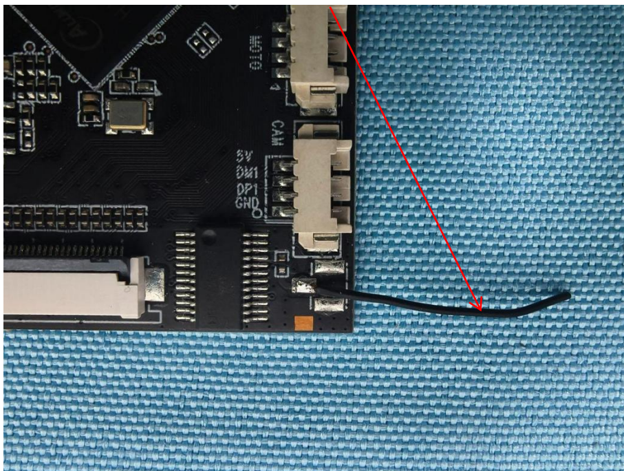
(Mainboard) BT-ANT
