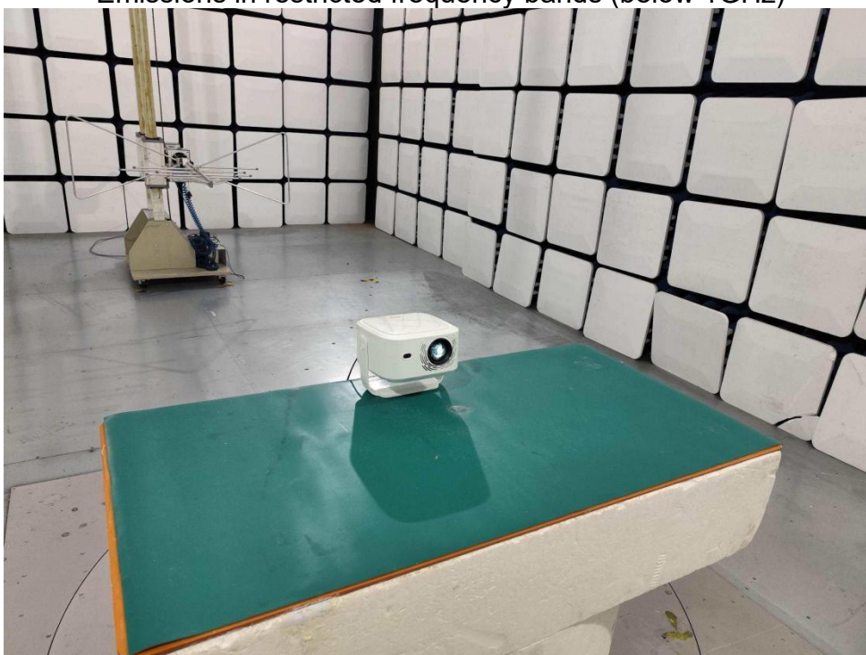
Emissions in restricted frequency bands (below 1GHz)
