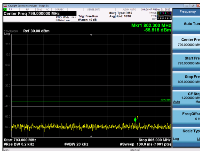
Band13-5MHz-16QAM-23205-1RB#0-Range4:793~805MHz
