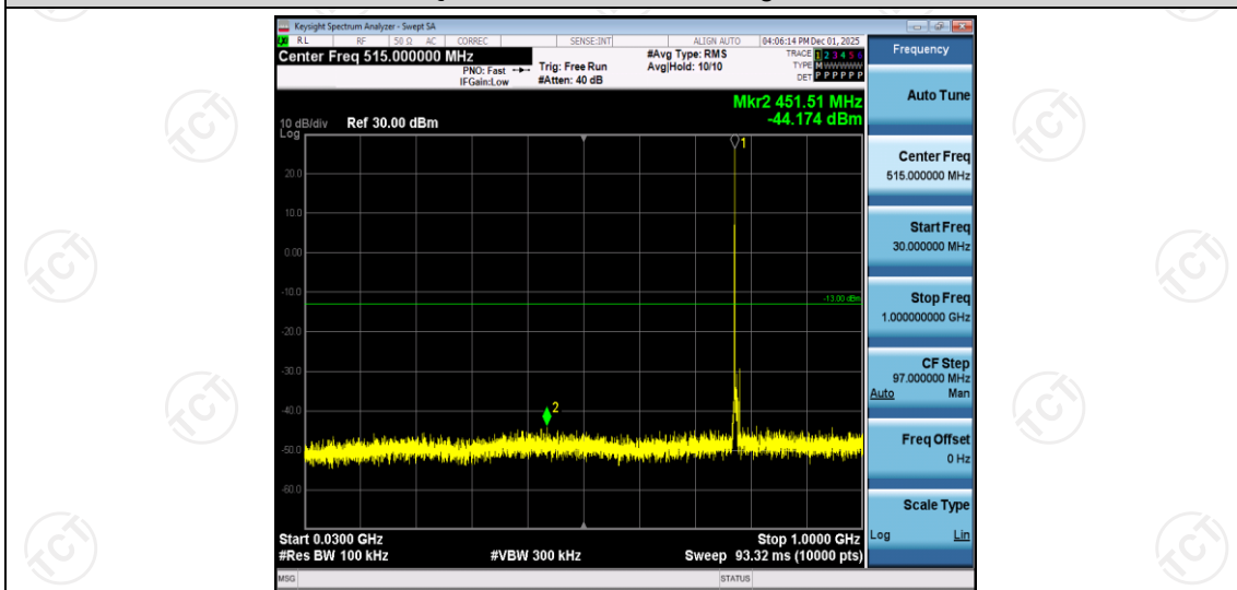
Band13-5MHz-16QAM-23205-1RB#0-Range1:30~1000MHz
