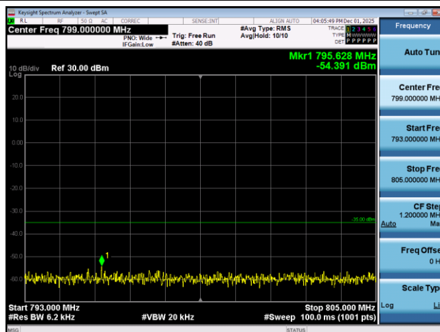
Band13-5MHz-QPSK-23205-1RB#0-Range4:793~805MHz
