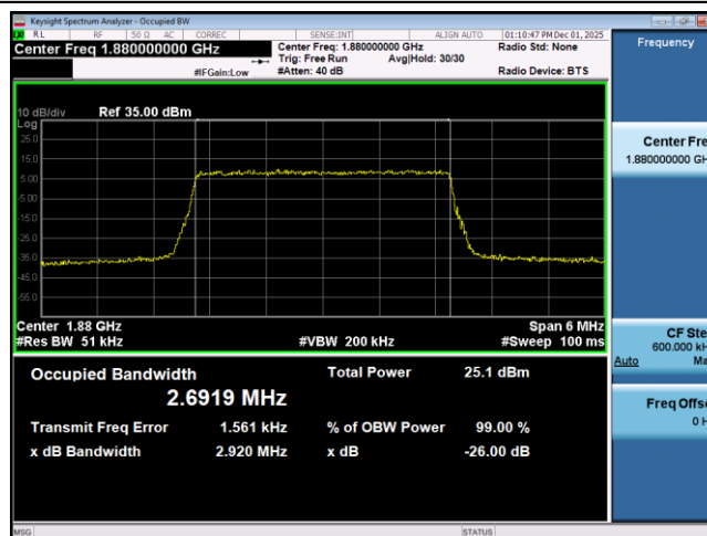
Band2-3MHz-16QAM-18900-15RB#0
