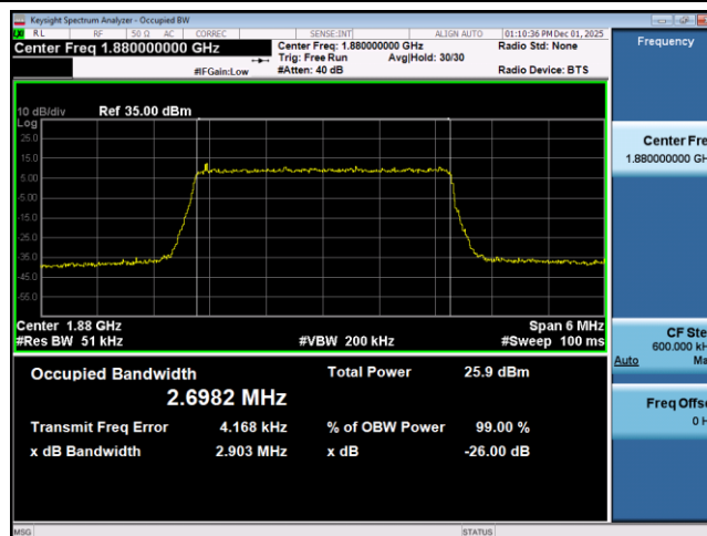
Band2-3MHz-QPSK-18900-15RB#0
