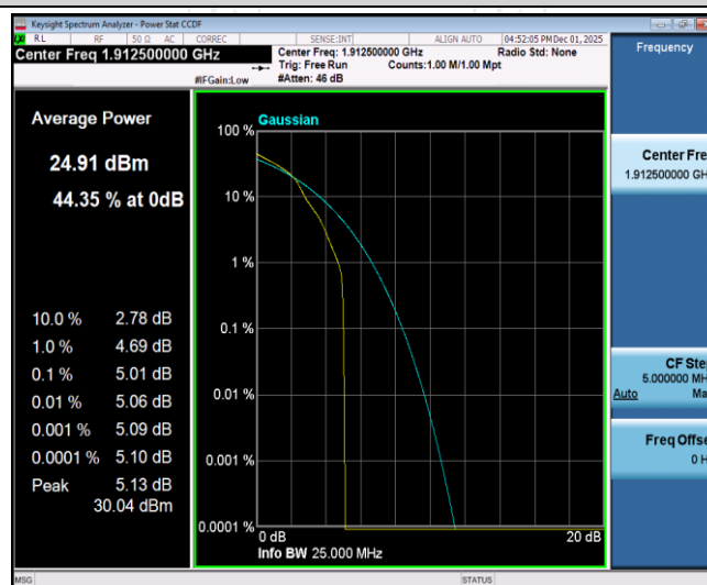
Band25-5MHz-16QAM-26665-1RB#0
