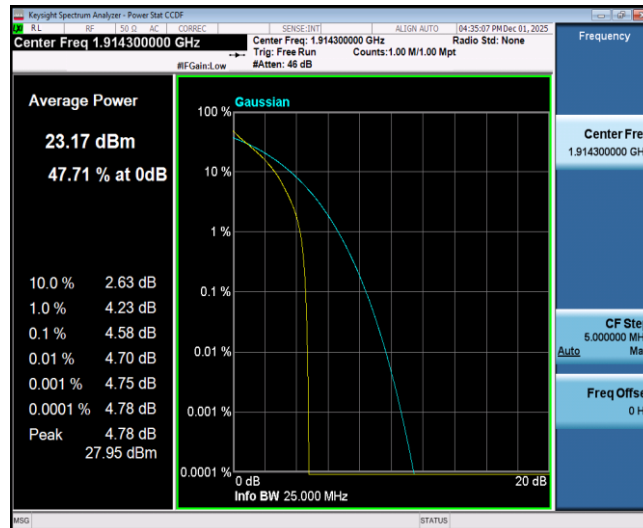
Band25-1.4MHz-QPSK-26683-6RB#0
