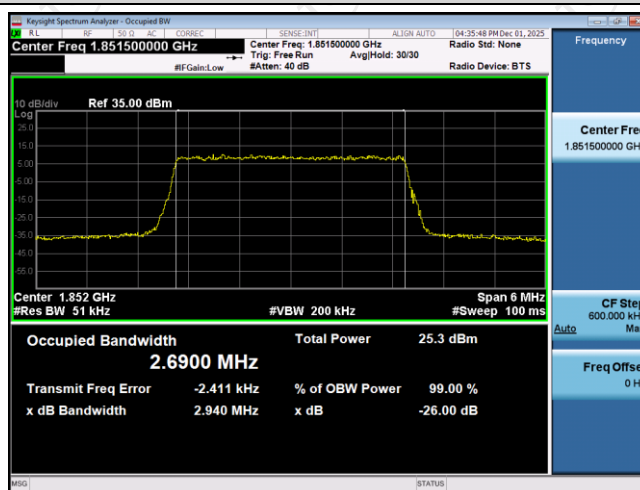
Band25-3MHz-16QAM-26055-15RB#0
