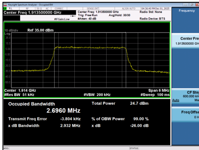
Band25-3MHz-16QAM-26675-15RB#0
