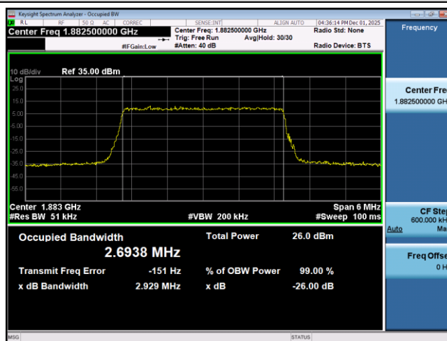
Band25-3MHz-16QAM-26365-15RB#0
