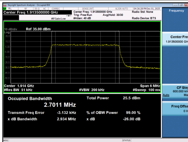
Band25-3MHz-QPSK-26675-15RB#0
