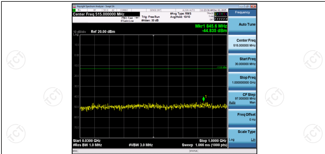
Band25-1.4MHz-QPSK-26047-1RB#0-Range1:30~1000MHz
