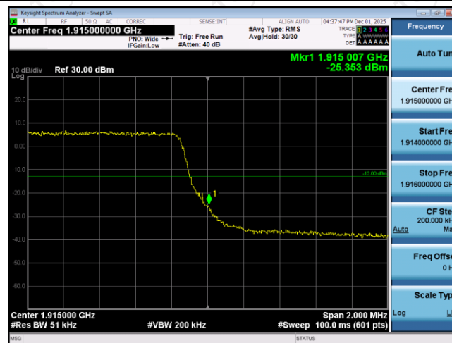
Band25-3MHz-16QAM-26675-15RB#0
