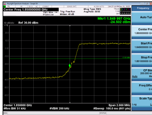
Band25-3MHz-16QAM-26055-15RB#0
