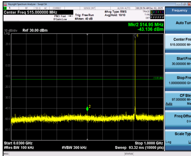
Band26-1.4MHz-16QAM-26740-1RB#0-Range1:30~1000MHz
