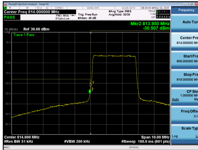
Band26-3MHz-16QAM-26705-15RB#0
