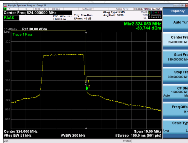
Band26-3MHz-16QAM-26775-15RB#0
