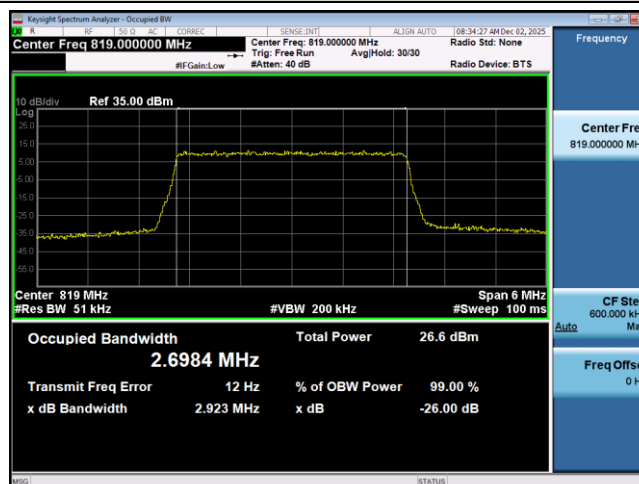
Band26-3MHz-QPSK-26740-15RB#0
