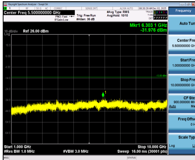
Band26-1.4MHz-QPSK-26783-1RB#0-Range2:1000~10000MHz
