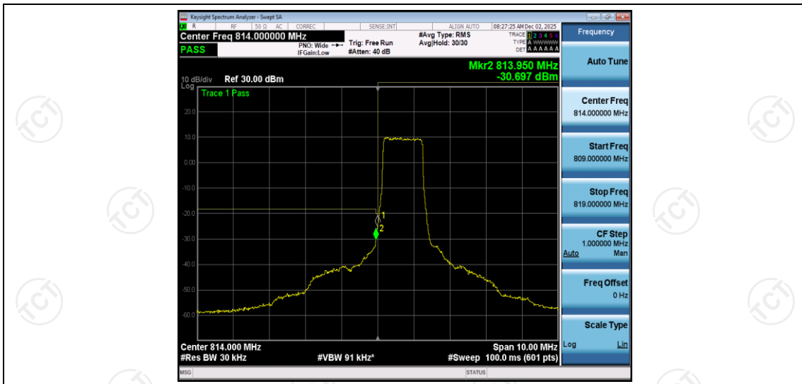
Band26-1.4MHz-QPSK-26697-6RB#0
