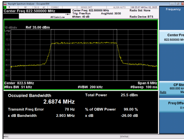
Band26-3MHz-16QAM-26775-15RB#0
