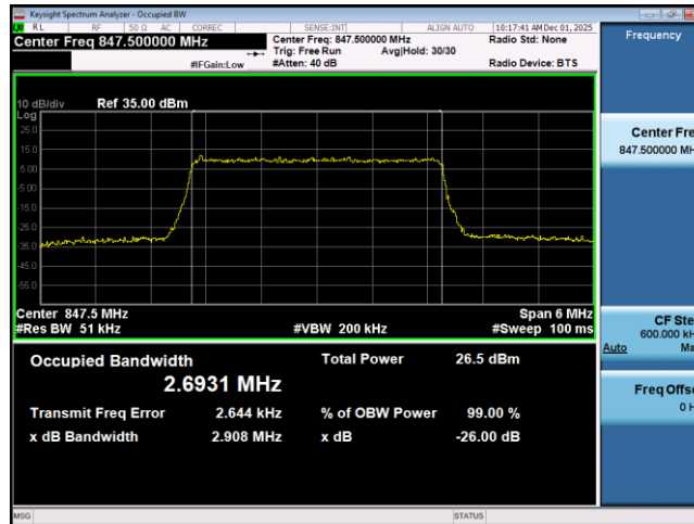
Band26-3MHz-QPSK-27025-15RB#0
