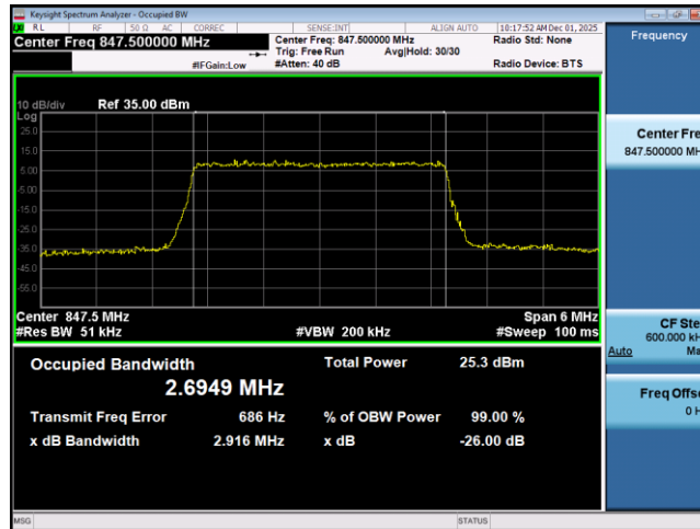
Band26-3MHz-16QAM-27025-15RB#0
