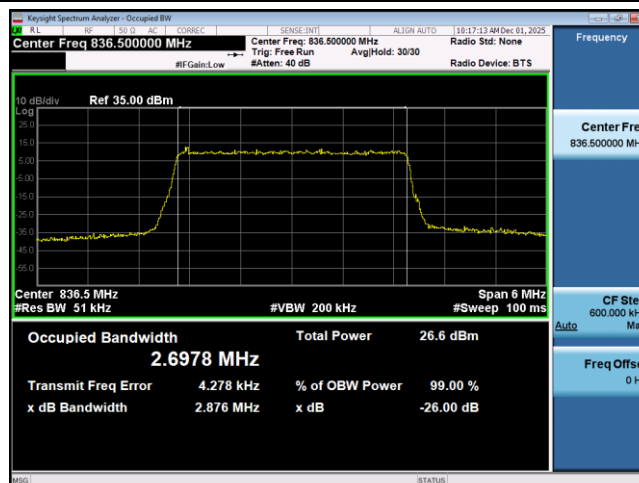
Band26-3MHz-QPSK-26915-15RB#0
