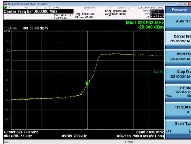
Band26-3MHz-16QAM-26805-15RB#0
