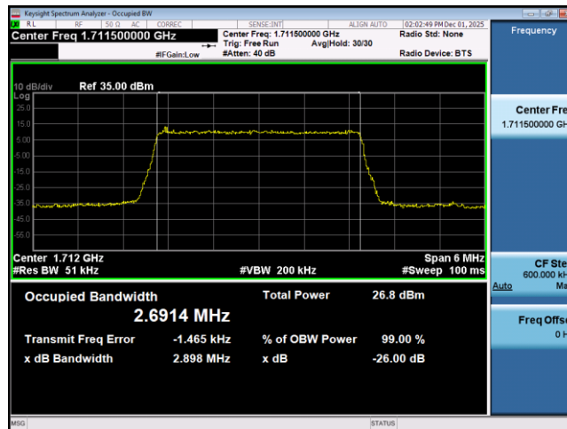
Band4-3MHz-QPSK-19965-15RB#0
