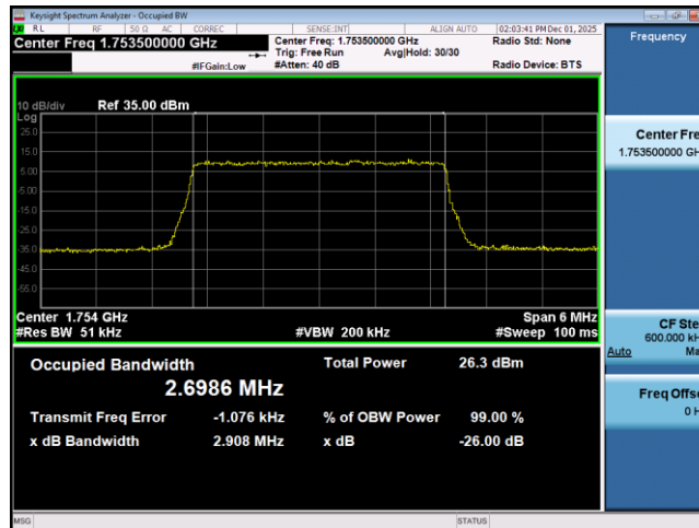
Band4-3MHz-QPSK-20385-15RB#0
