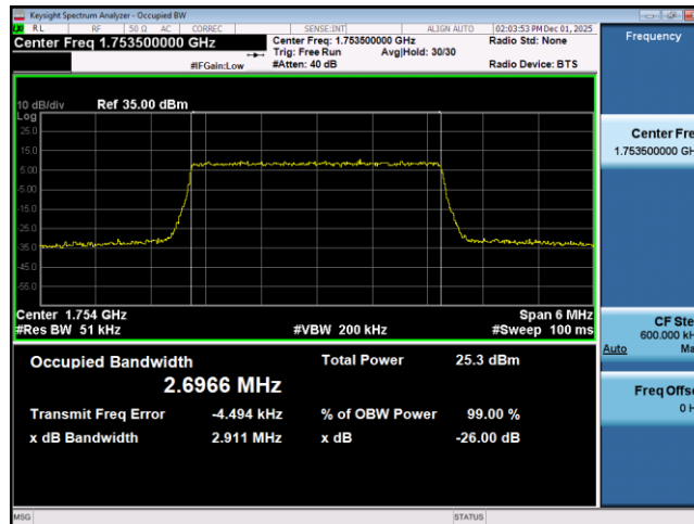
Band4-3MHz-16QAM-20385-15RB#0
