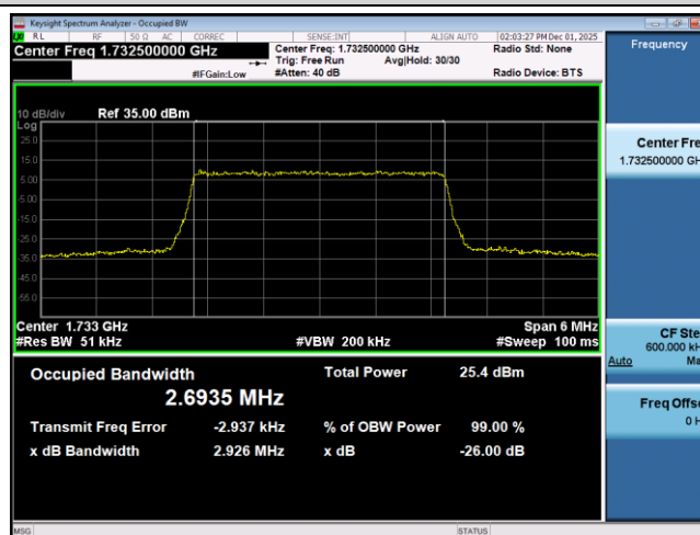
Band4-3MHz-16QAM-20175-15RB#0
