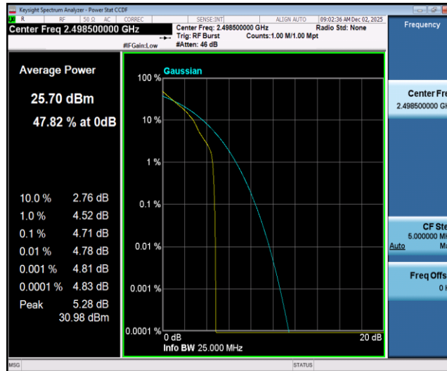
Band41-5MHz-QPSK-39675-1RB#0
