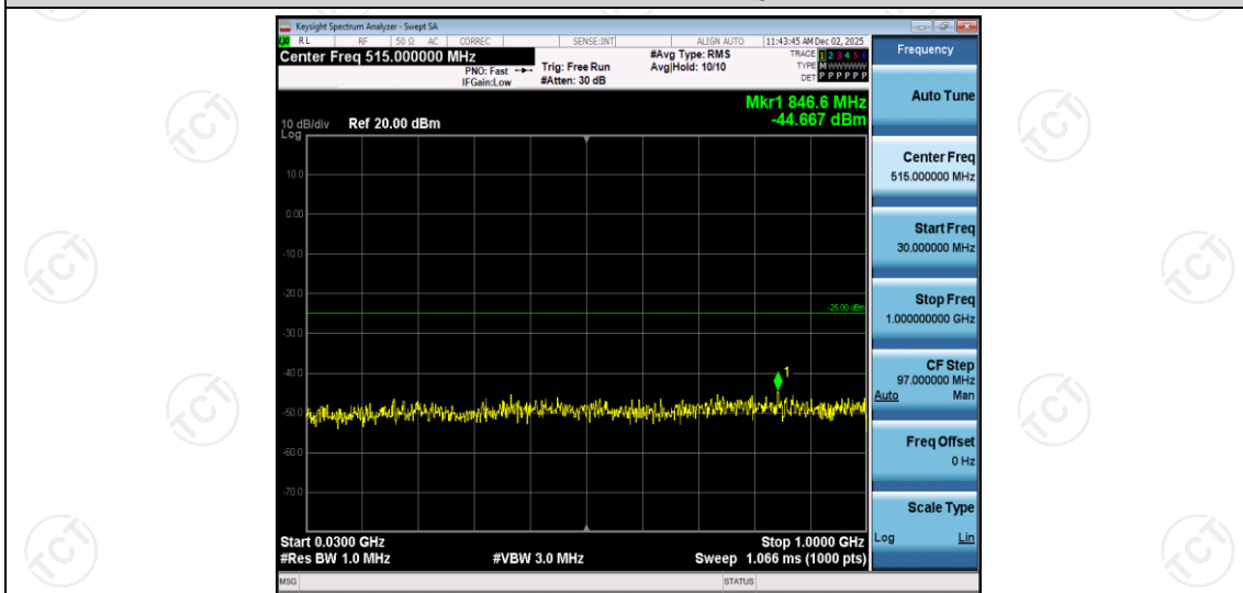
Band41-5MHz-16QAM-39675-1RB#0-Range1:30~1000MHz
