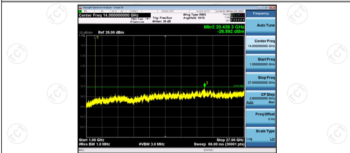
Band41-5MHz-16QAM-39675-1RB#0-Range2:1000~27000MHz
