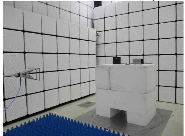
FCC_15_249_Radiated_External antenna_Setup
