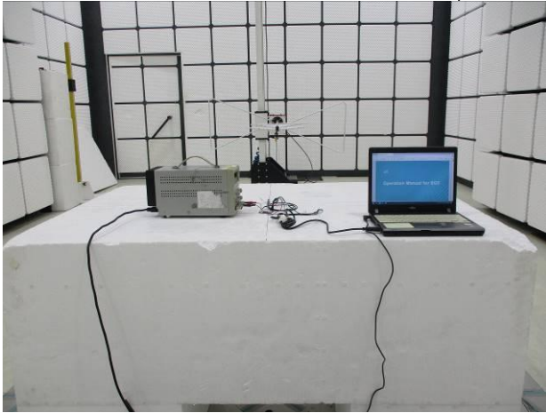
FCC_15_249_Radiated_External antenna_Setup
