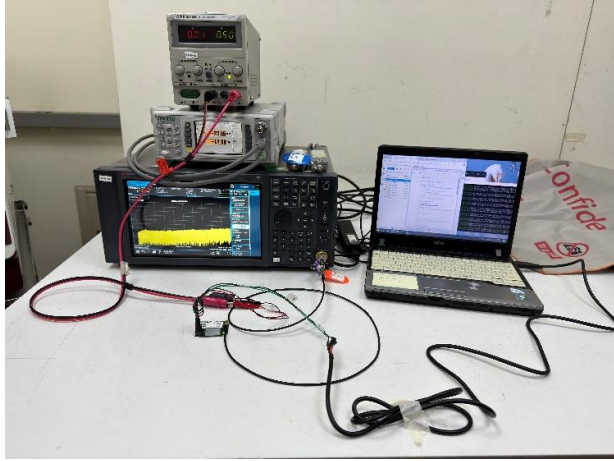
FCC_15_247_Radiated_External antenna_Setup
