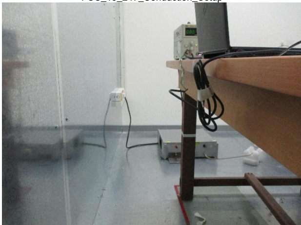
FCC_15_249_Conduction_Setup
