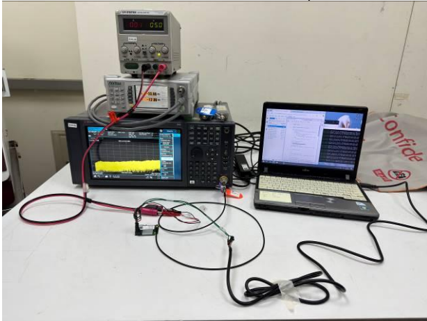
FCC_15_249_Conducted_Setup
