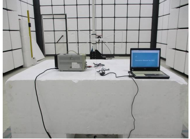
FCC_15_249_Radiated_Internal antenna_Setup
