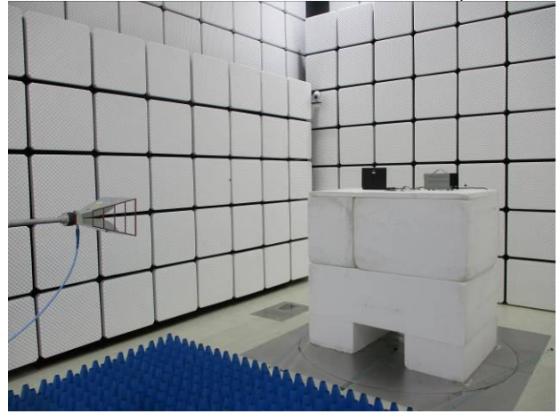
FCC_15_249_Radiated_Internal antenna_Setup
