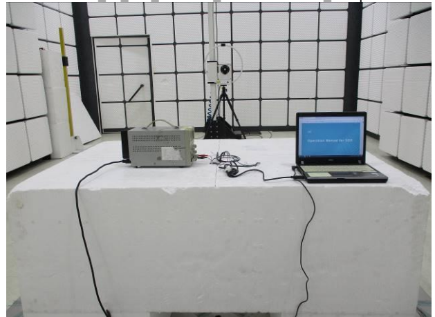
FCC_15_247_Radiated_External antenna_Setup
