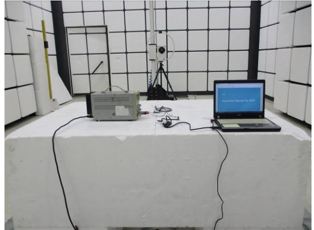
FCC_15_249_Radiated_External antenna_Setup
