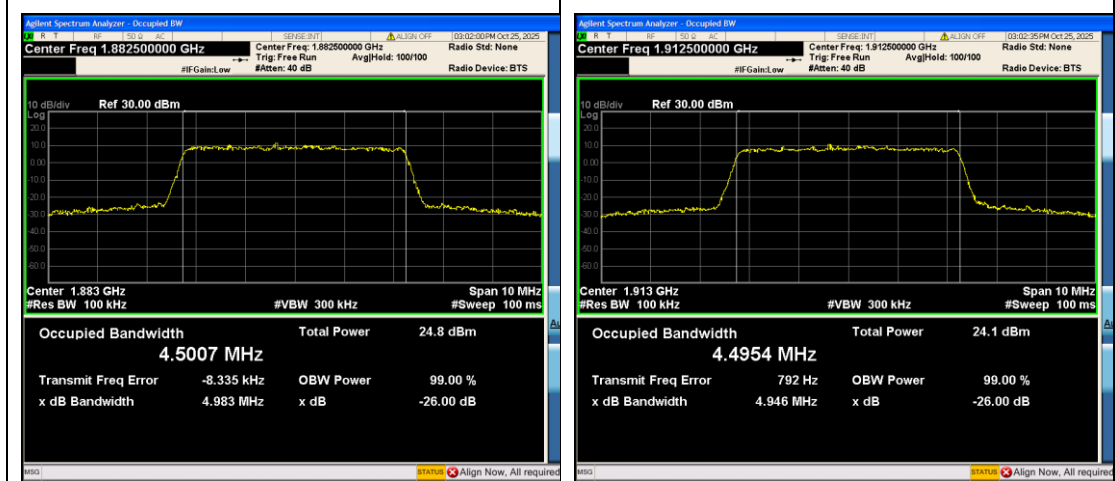
Band25-5MHz-16QAM-26365-25RB#0-PASS
