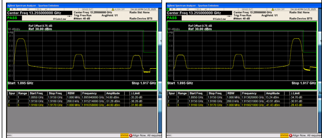
Band25_20MHz_16QAM_26590_1RB#0
