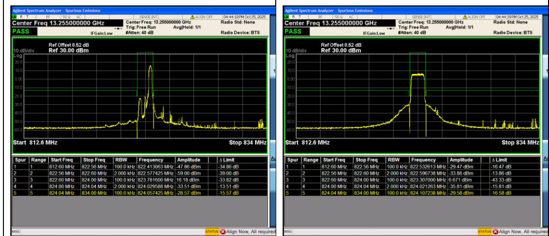
Band26_1.4MHz_16QAM_26783_1RB#5
