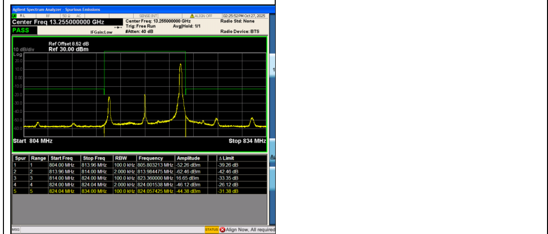
Band26_10MHz_16QAM_26740_1RB#49
