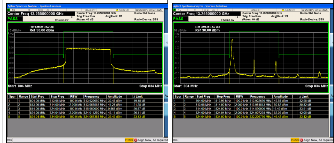
Band26_10MHz_QPSK_26740_50RB#0
