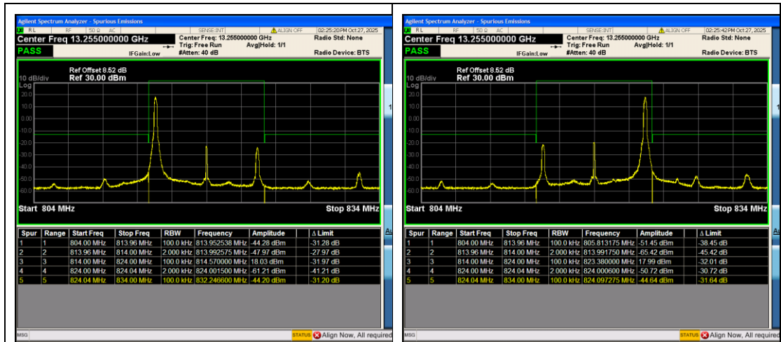
Band26_10MHz_QPSK_26740_1RB#0
