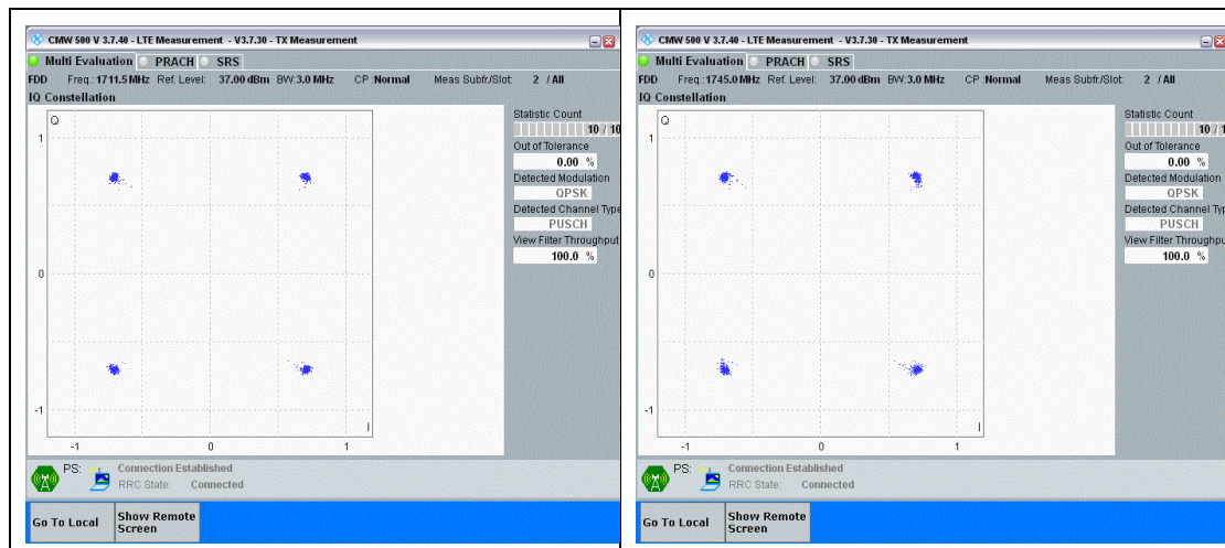
Band66-3MHz-QPSK-131987-15RB#0-PASS
