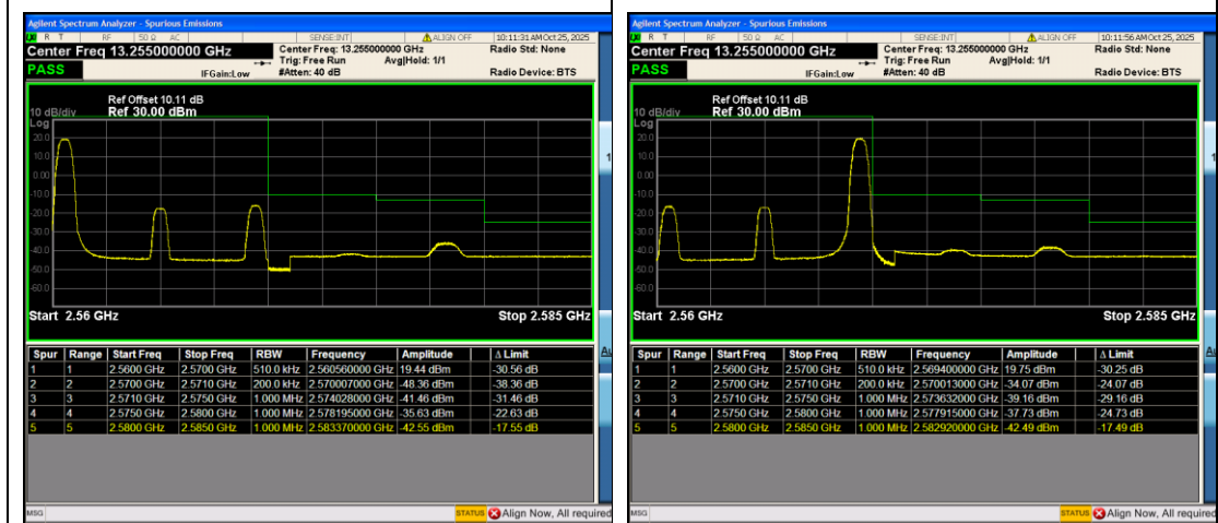
Band7_10MHz_16QAM_21400_1RB#0
