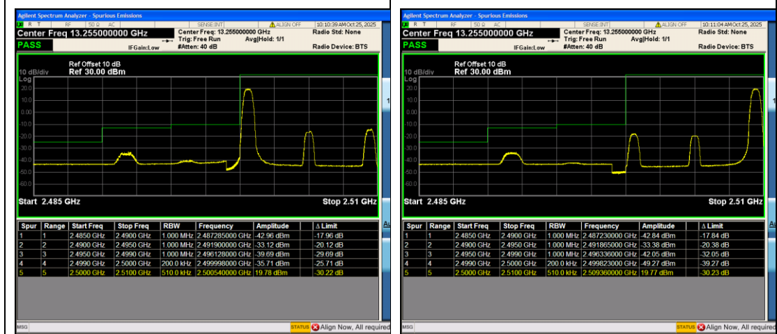
Band7_10MHz_16QAM_20800_1RB#0
