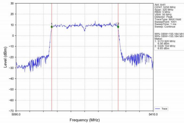
802.11ax(HEW160)_MCH_5250MHz_SU_/_Ant1_NTNV
