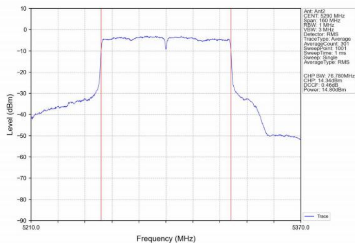
802.11ax(HEW80)_MCH_5290MHz_SU_/_Ant2_NTNV
