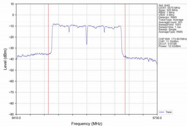
802.11ac(VHT160)_MCH_5570MHz_Ant2_NTNV
