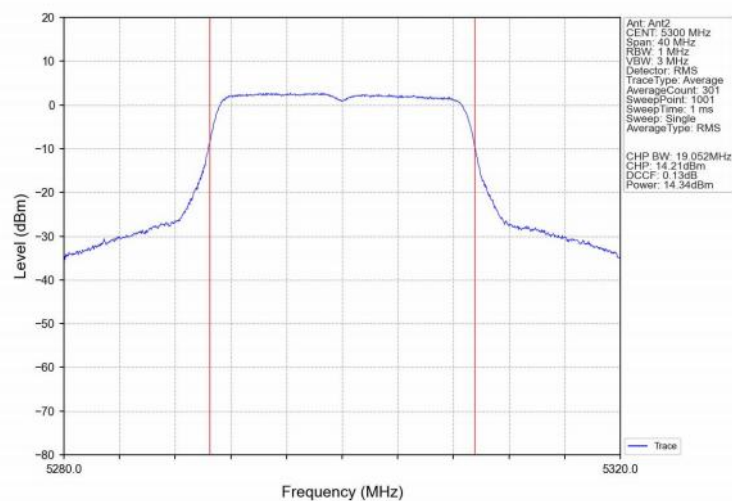
802.11ax(HEW20)_MCH_5300MHz_SU_/_Ant2_NTNV
