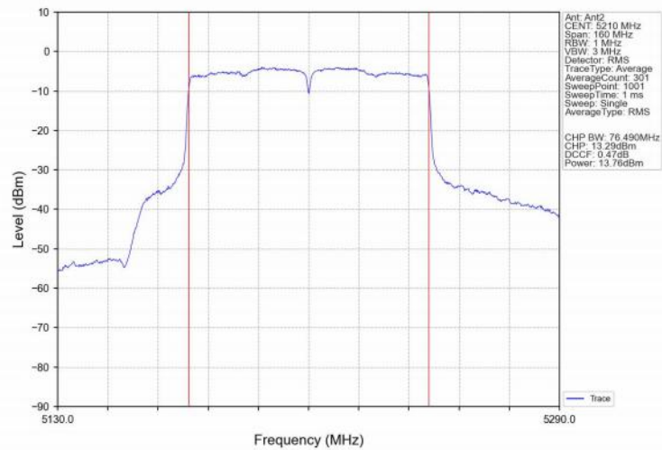
802.11ax(HEW80)_MCH_5210MHz_SU_/_Ant2_NTNV
