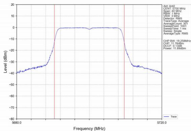
802.11ax(HEW20)_HCH_5700MHz_SU_/_Ant2_NTNV
