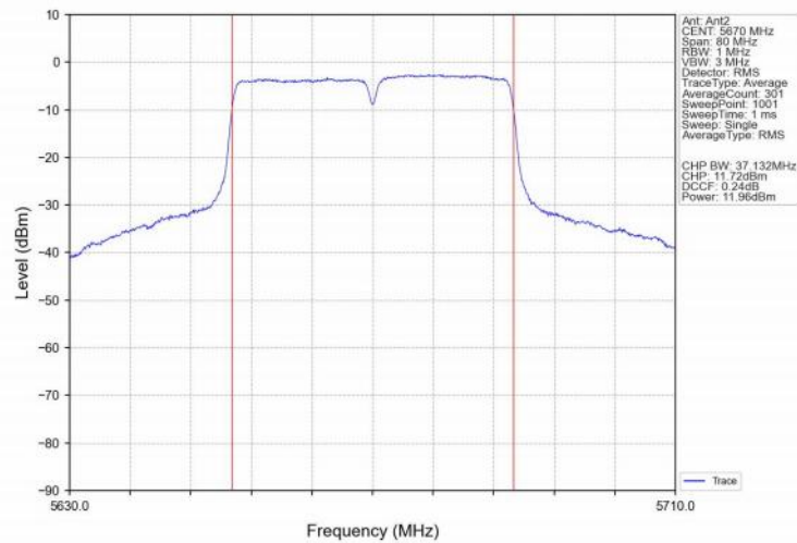
802.11ax(HEW40)_HCH_5670MHz_SU_/_Ant2_NTNV
