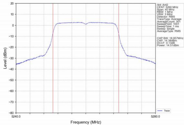
802.11ax(HEW20)_LCH_5260MHz_SU_ / Ant2_NTNV
