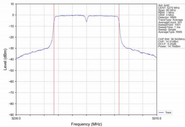
802.11ax(HEW40)_LCH_5270MHz_SU_ / Ant2_NTNV
