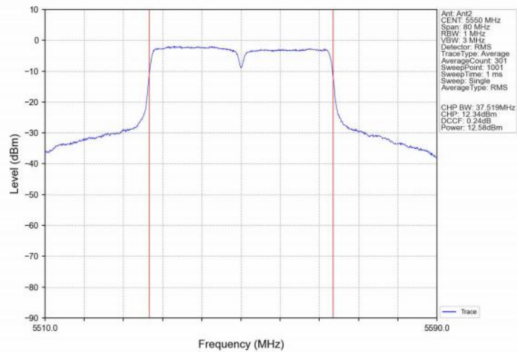
802.11ax(HEW40)_MCH_5550MHz_SU_/_Ant2_NTNV
