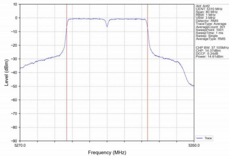
802.11ax(HEW40)_HCH_5310MHz_SU_/_Ant2_NTNV
