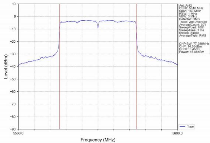
802.11ax(HEW80)_HCH_5610MHz_SU_/_Ant2_NTNV
