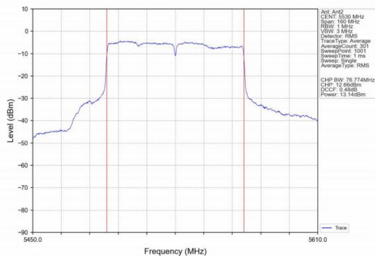
802.11ax(HEW80)_LCH_5530MHz_SU_ / Ant2_NTNV
