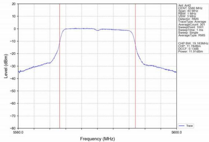
802.11ax(HEW20)_MCH_5580MHz_SU_/_Ant2_NTNV
