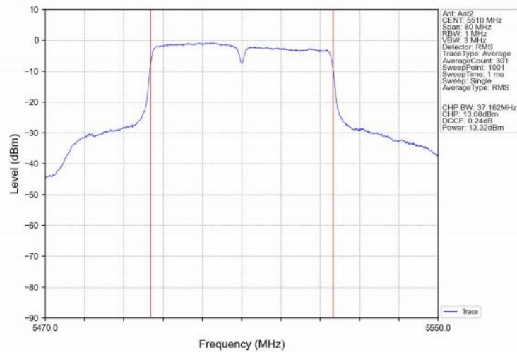
802.11ax(HEW40)_LCH_5510MHz_SU_ / Ant2_NTNV
