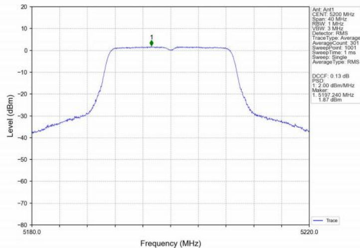
802.11ax(HEW20)_MCH_5200MHz_SU_/_Ant1_NTNV
