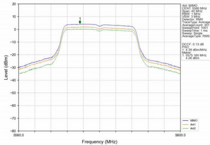
802.11ax(HEW20)_MCH_5580MHz_SU_/_MIMO_NTNV
