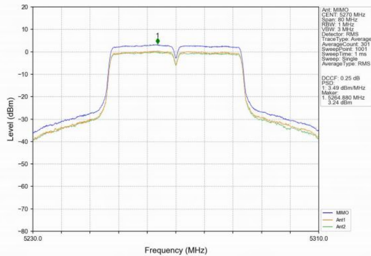
802.11ax(HEW40)_LCH_5270MHz_SU_ / MIMO_NTNV
