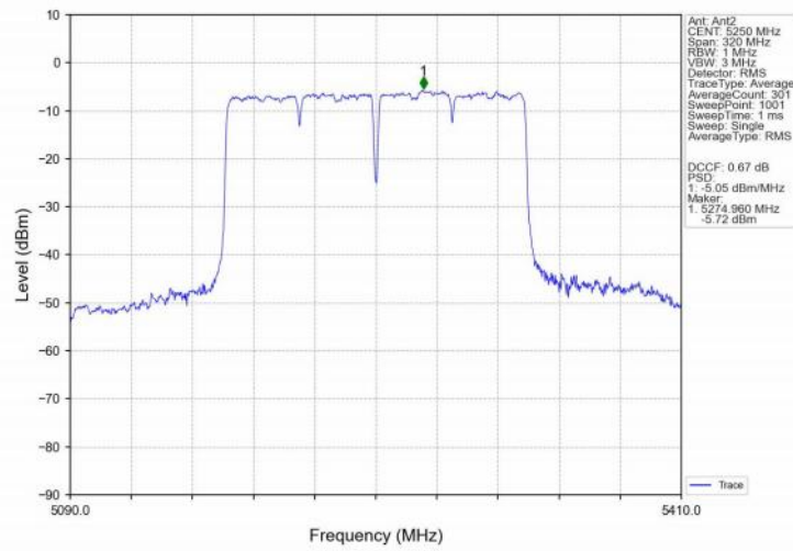
802.11ac(VHT160)_MCH_5250MHz_MIMO_NTNV
