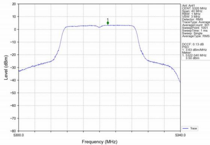
802.11ax(HEW20)_HCH_5320MHz_SU_/_Ant1_NTNV
