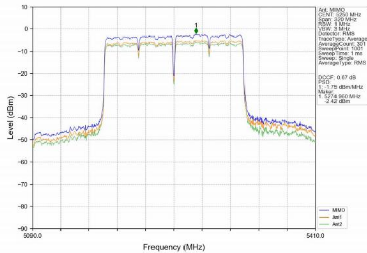
802.11ac(VHT160)_MCH_5250MHz_MIMO_NTNV
