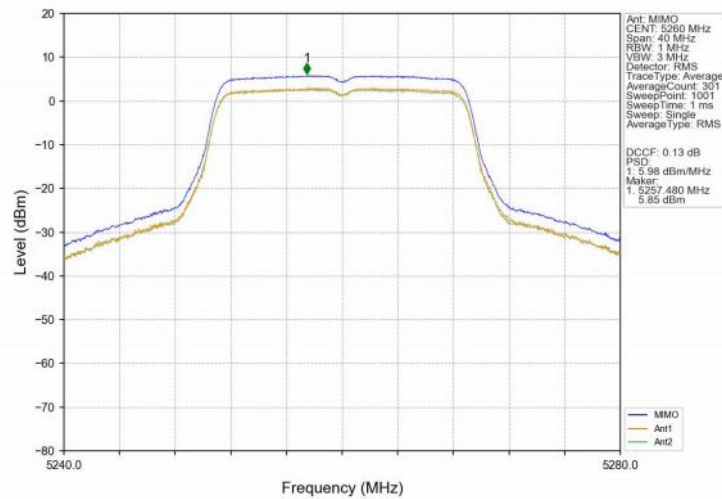
802.11ax(HEW20)_LCH_5260MHz_SU_ / MIMO_NTNV
