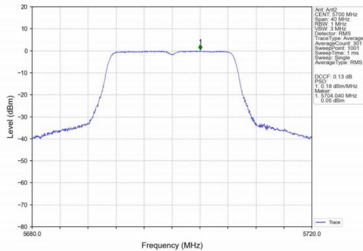
802.11ax(HEW20)_HCH_5700MHz_SU_/_Ant2_NTNV
