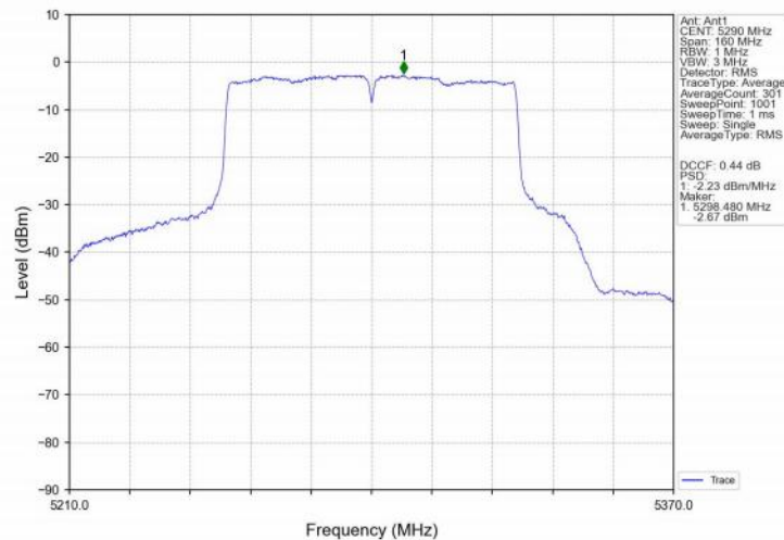
802.11ac(VHT80)_MCH_5290MHz_Ant1_NTNV
