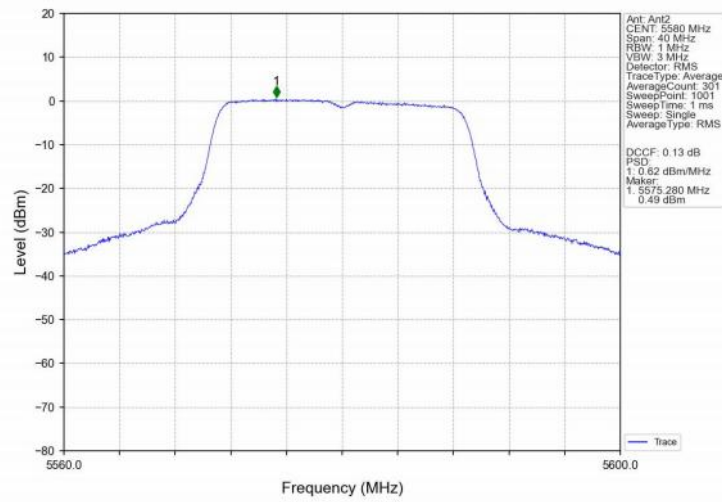
802.11ax(HEW20)_MCH_5580MHz_SU_/_MIMO_NTNV
