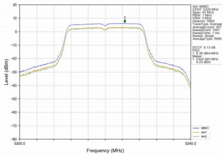
802.11ax(HEW20)_HCH_5320MHz_SU_/_MIMO_NTNV
