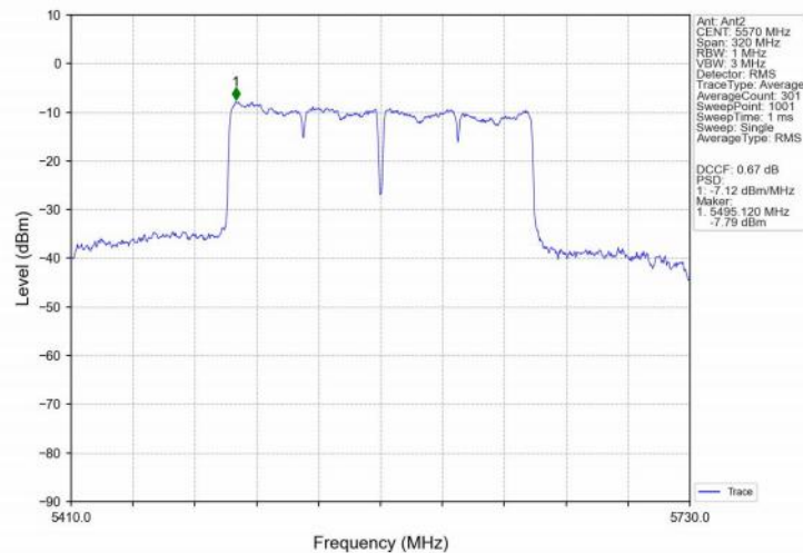
802.11ac(VHT160)_MCH_5570MHz_Ant2_NTNV
