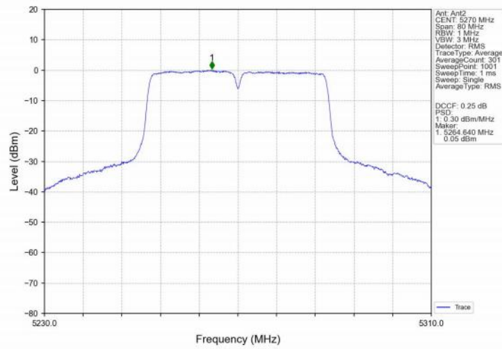
802.11ax(HEW40)_LCH_5270MHz_SU_ / MIMO_NTNV
