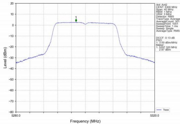
802.11ax(HEW20)_MCH_5300MHz_SU_/_Ant2_NTNV
