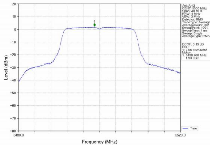
802.11ax(HEW20)_LCH_5500MHz_SU_ / Ant2_NTNV
