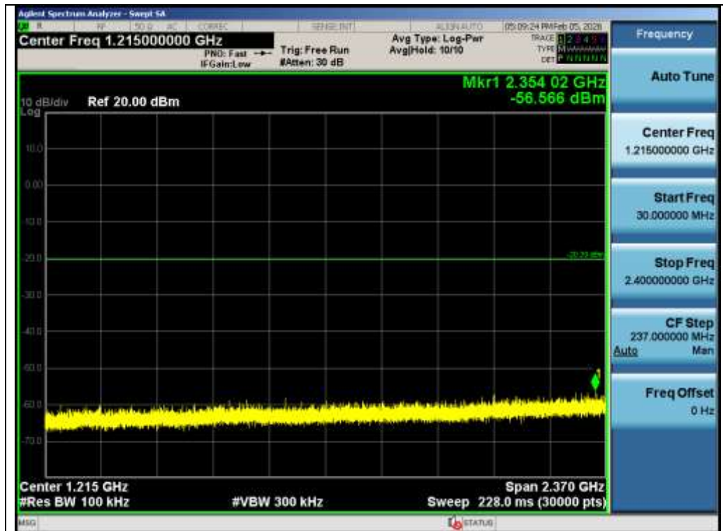
Test_Graph_2.4G_ANT1_2430_GFSK_Lower Band Emissions
