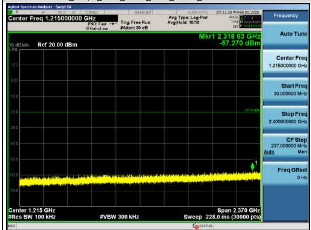
Test_Graph_2.4G_ANT1_2476_GFSK_Lower Band Emissions
