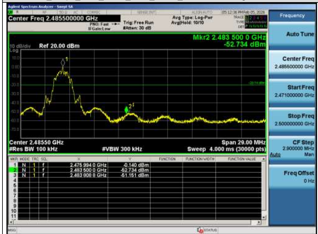
Test_Graph_2.4G_ANT1_2476_GFSK_Higher Band Edge Emissions
