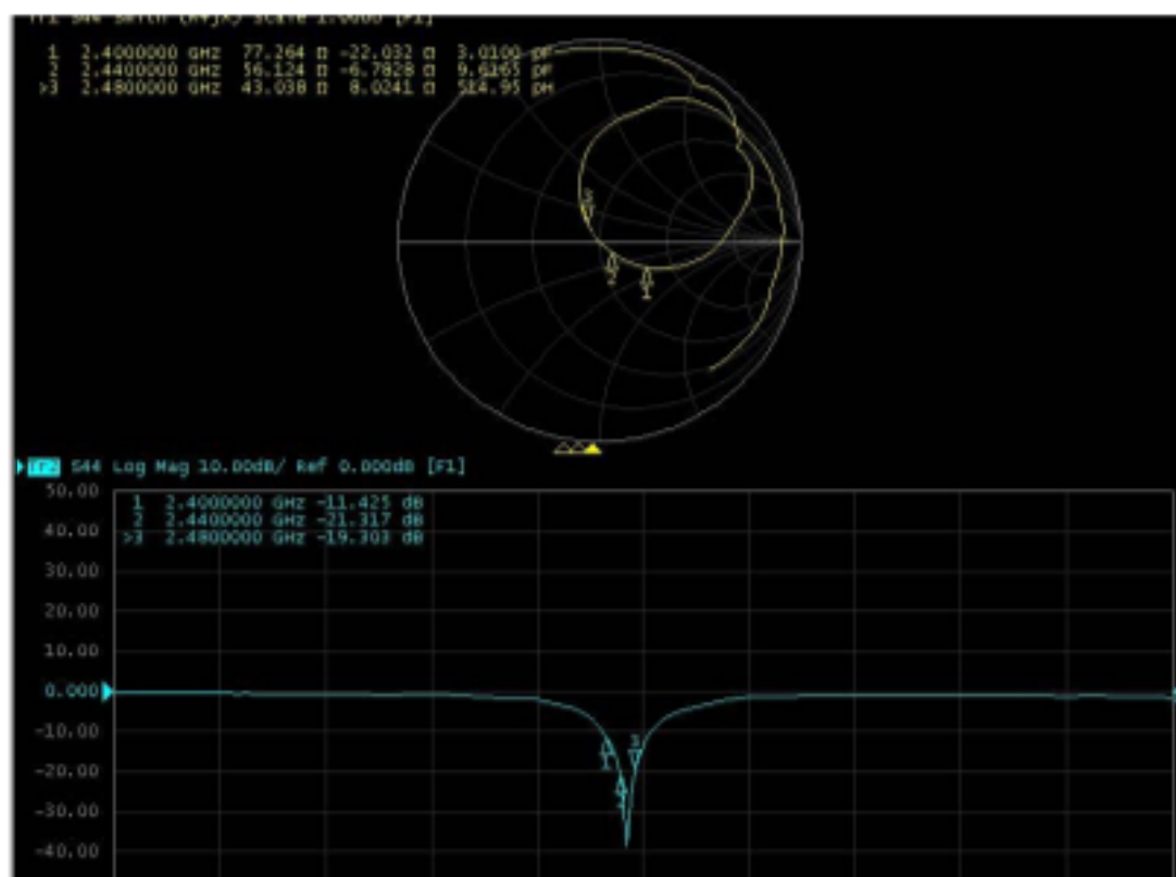
Return Loss
