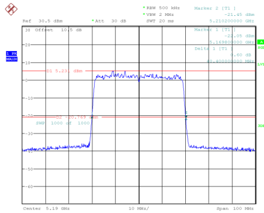
802.11ax40_5190MHz_RU_Full
