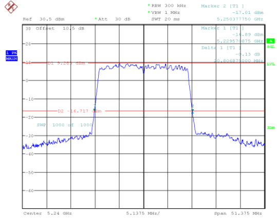
802.11ax20_5240MHz_RU_Full
