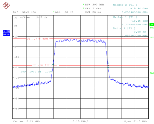
802.11ax20_5240MHz_RU_Full
