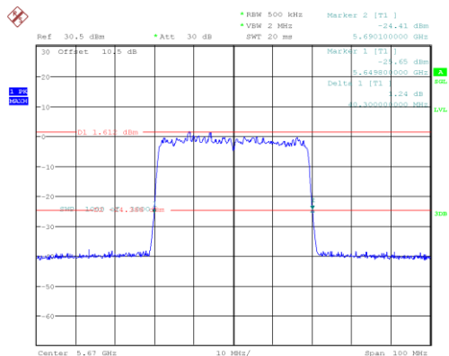
802.11ax40_5670MHz_RU_Full
