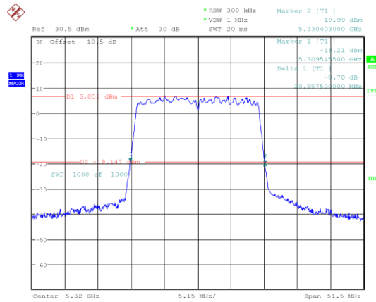
802.11ax20_5320MHz_RU_Full
