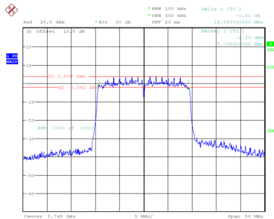
802.11ax20_5745MHz_RU_Full
