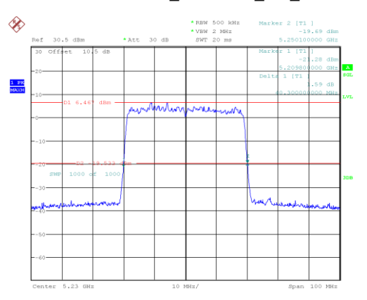
802.11ax40_5230MHz_RU_Full
