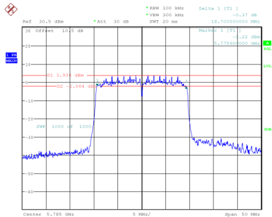
802.11ax20_ 5785MHz_RU_Full
