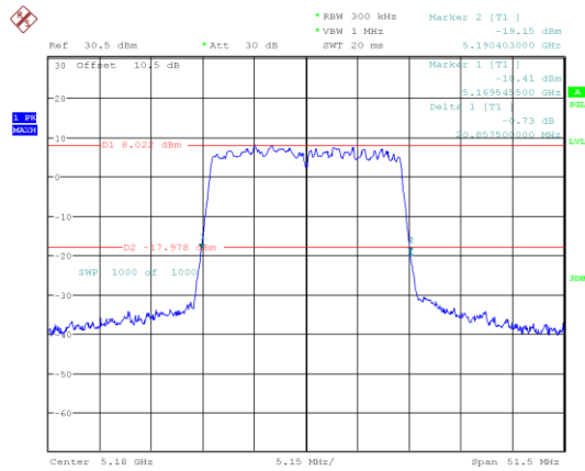
802.11ax20_5180MHz_RU_Full
