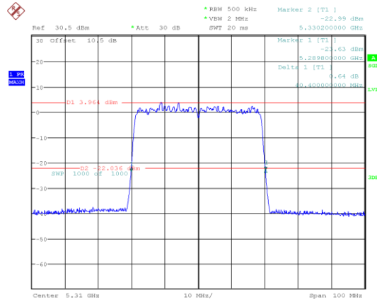
802.11ax40_5310MHz_RU_Full
