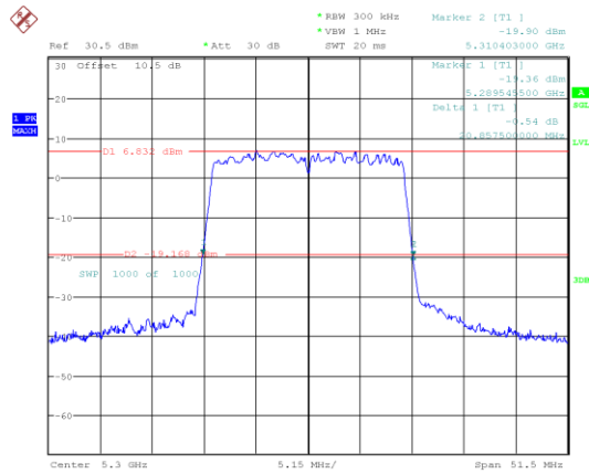
802.11ax20_5300MHz_RU_Full
