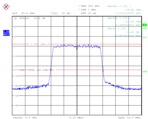
802.11ax20_5500MHz_RU_Full
