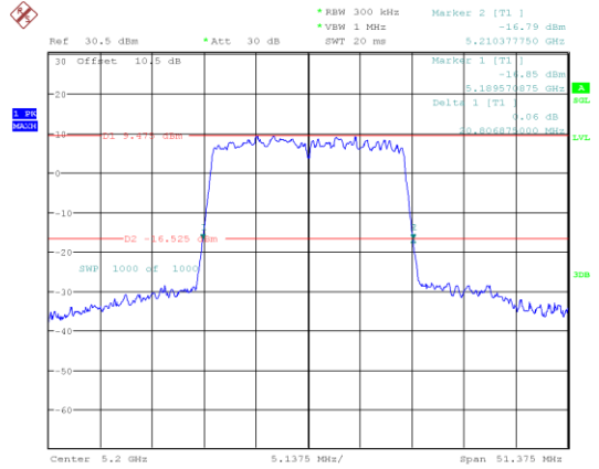
802.11ax20_5200MHz_RU_Full
