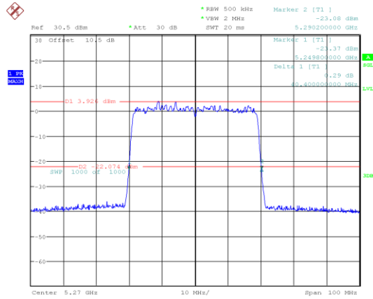
802.11ax40_5270MHz_RU_Full
