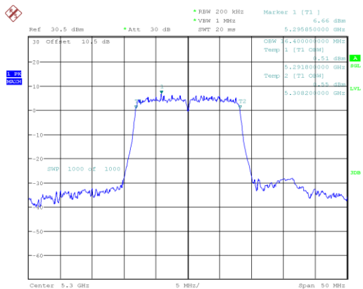
802.11a_5300MHz
