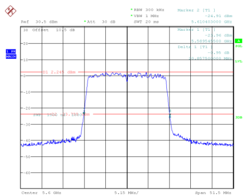
802.11ax20_5600MHz_RU_Full
