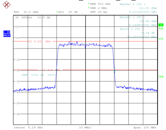
802.11ax40_5190MHz_RU_Full
