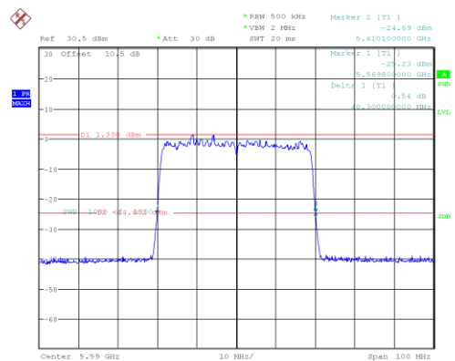
802.11ax40_5590MHz_RU_Full
