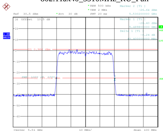
802.11ax40_5510MHz_RU_Full
