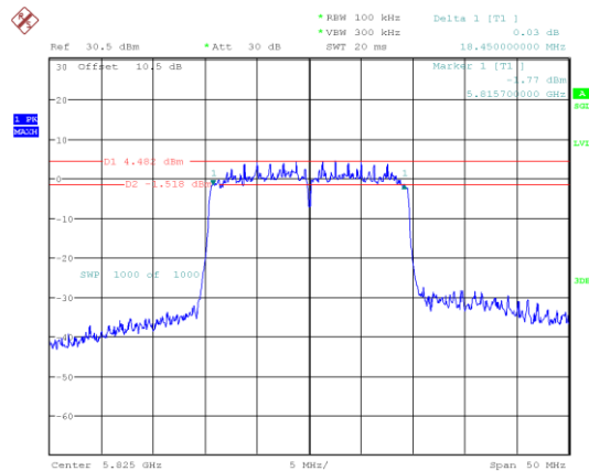
802.11ax20_ 5825MHz_RU_Full
