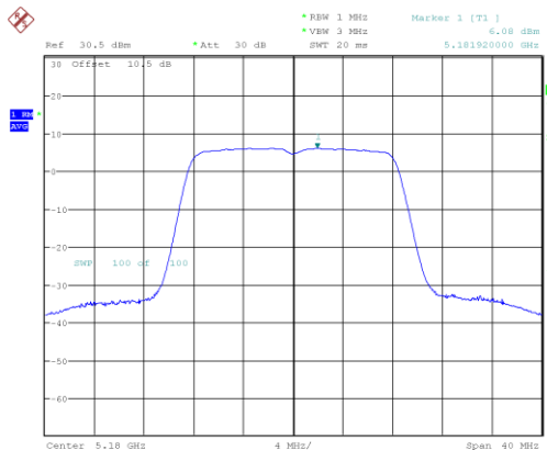
802.11a_5180MHz
