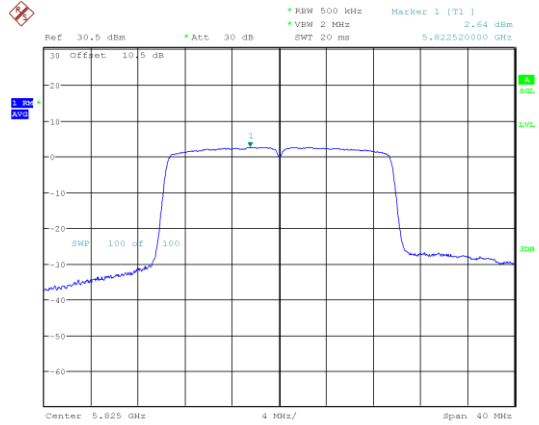
802.11ax20_5825MHz_RU_Full
