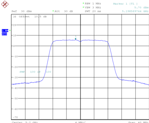
802.11a_5200MHz
