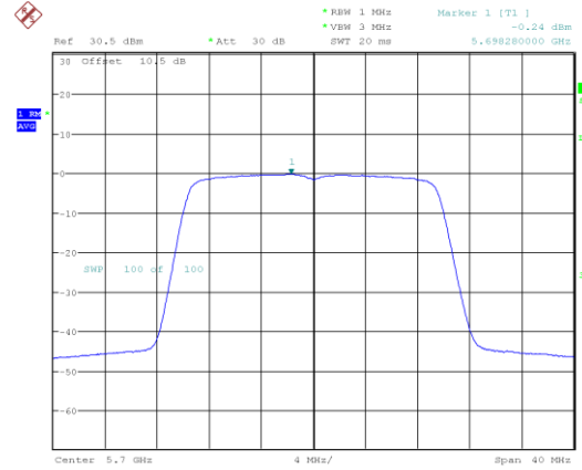
802.11ax20_5700MHz_RU_Full
