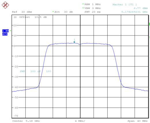
802.11ax20_5180MHz_RU_Full
