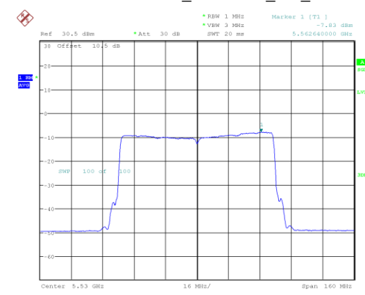
802.11ax80_5530MHz_RU_Full
