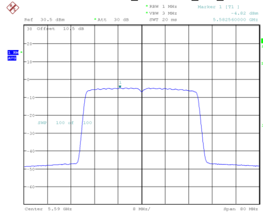
802.11ax40_5590MHz_RU_Full
