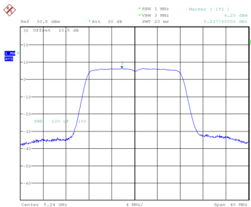
802.11a_5240MHz
