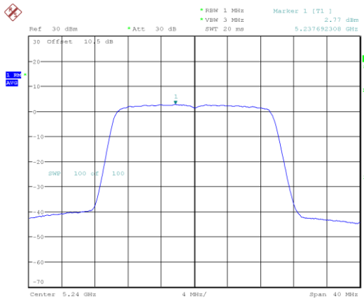
802.11ax20_5240MHz_RU_Full
