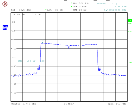
802.11ax80_5775MHz_RU_Full
