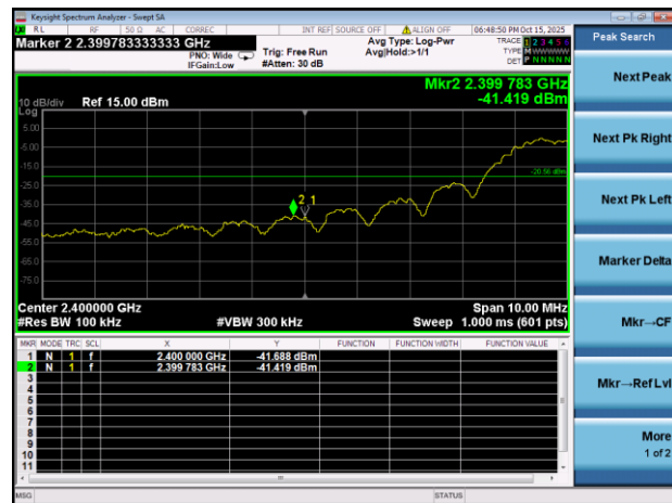
Zigbee LOW CHANNEL, BAND EDGE
