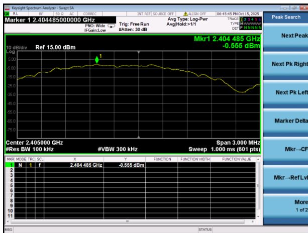
Zigbee LOW CHANNEL, CARRIER LEVEL
