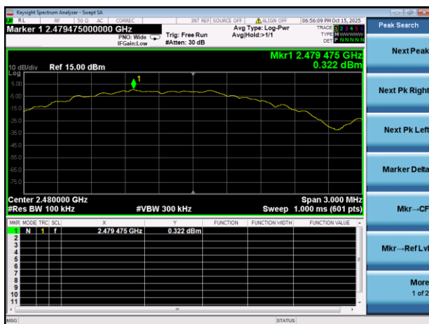
Zigbee HIGH CHANNEL, CARRIER LEVEL
