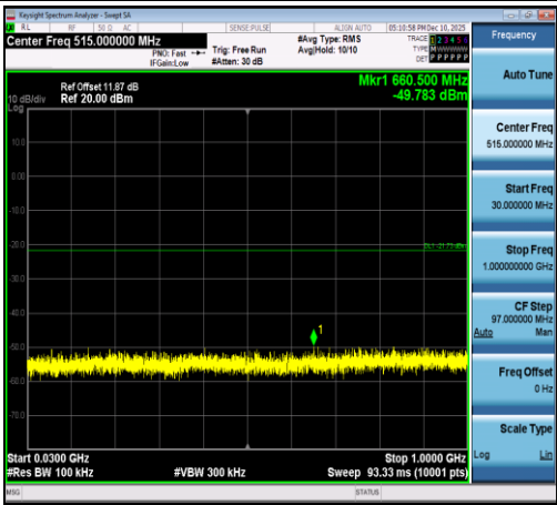
2.4GHz-Ant1-2480-30~1000-PASS
