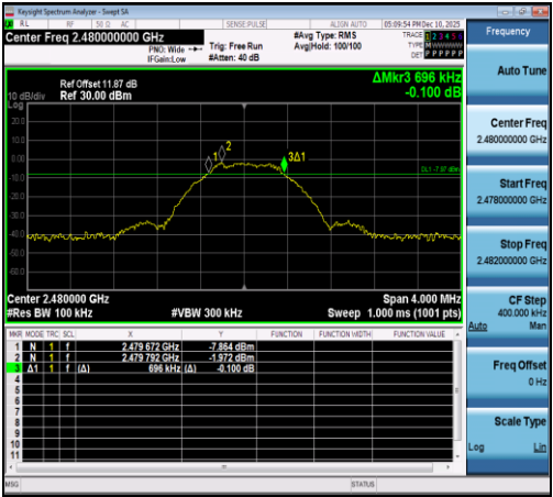
2.4GHz-Ant1-2480-PASS
