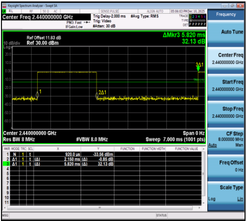
NTNV-2.4GHz-Ant1-2440
