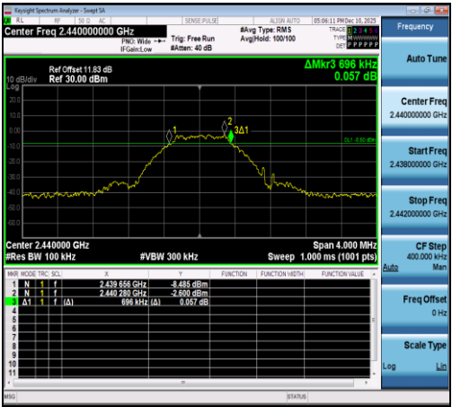
2.4GHz-Ant1-2440-PASS
