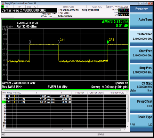
NTNV-2.4GHz-Ant1-2480
