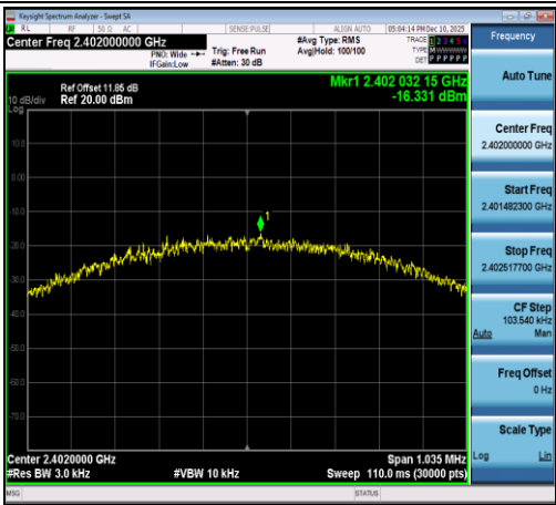
2.4GHz-Ant1-2402-PASS
