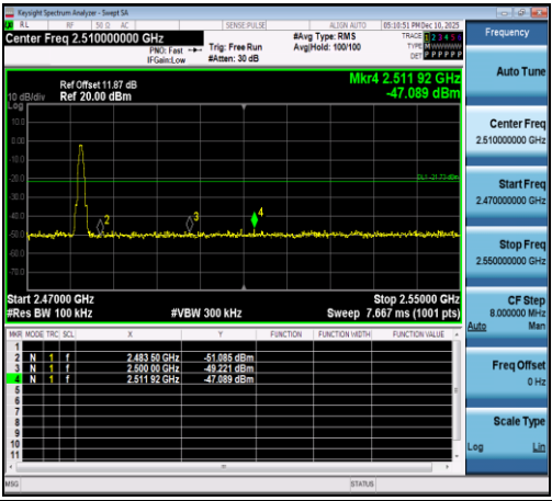
2.4GHz-Ant1-2480-PASS
