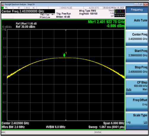
2.4GHz-Ant1-2402-PASS
