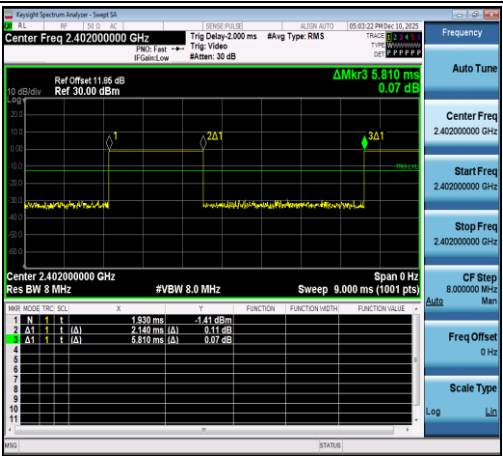
NTNV-2.4GHz-Ant1-2402
