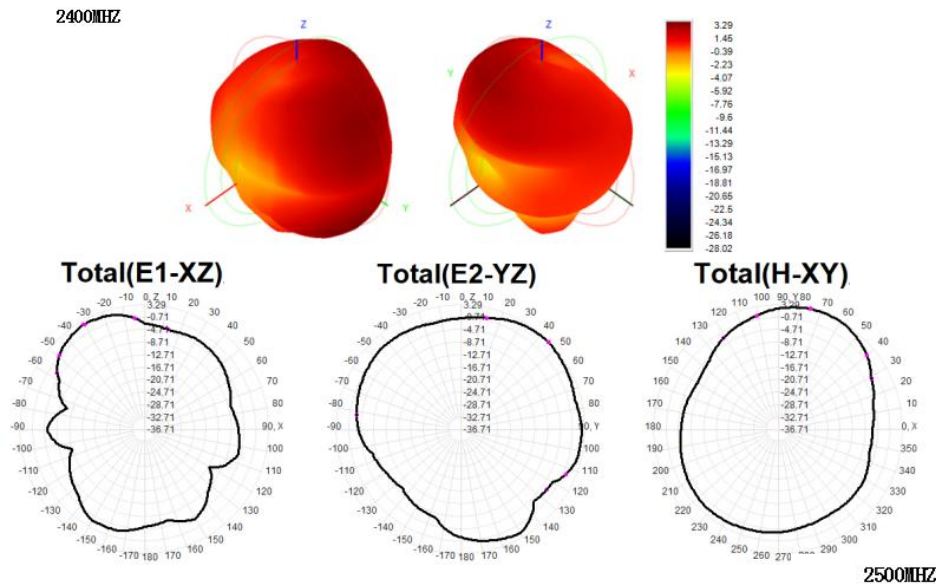
Radiation Patterns ( 2400MHz )
