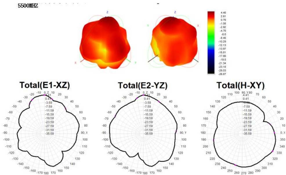
Radiation Patterns ( 5500MHz )
