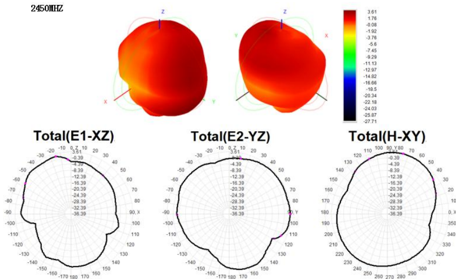
Radiation Patterns ( 2450MHz )
