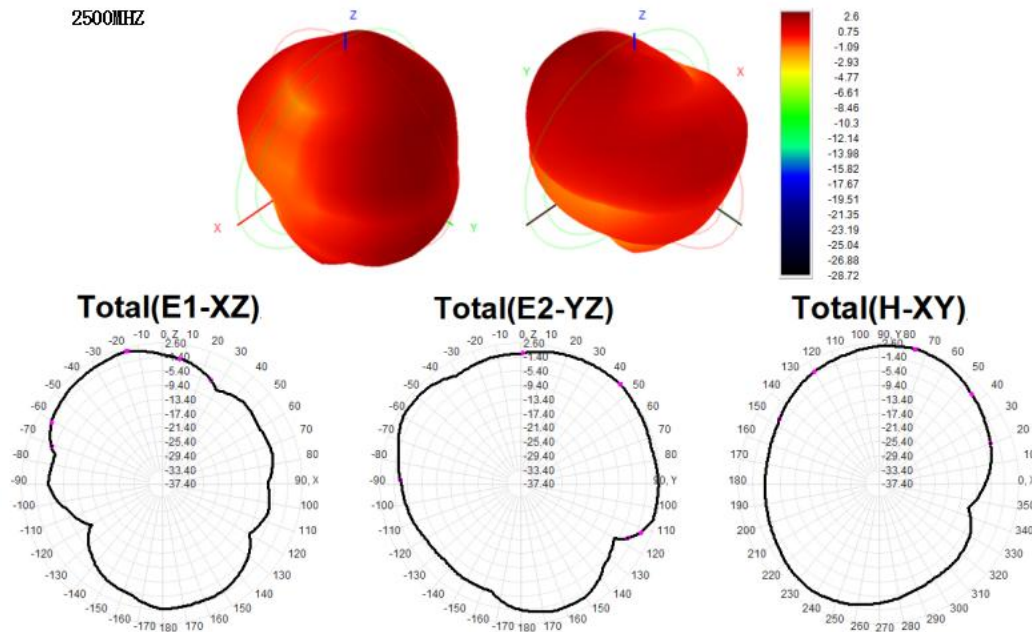
Radiation Patterns ( 2500MHz )
