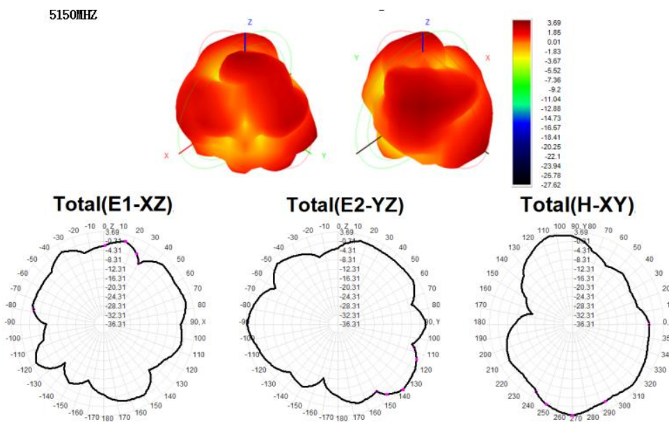
Radiation Patterns ( 5150MHz )
