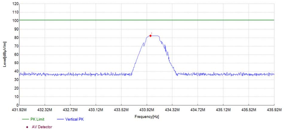
(Antenna Vertical)
