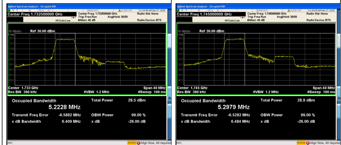
Band4-20MHz-16QAM-20175-27RB#0-PASS
