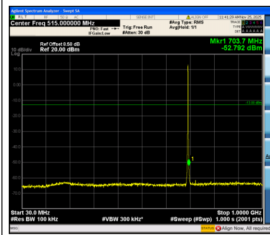
Band12_1.4MHz_QPSK_23017_6RB#0_30~1000_30~1000
