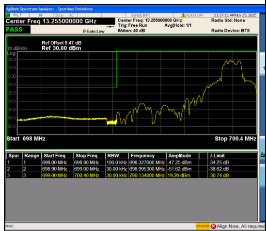
Band12_1.4MHz_16QAM_23017_1RB#5
