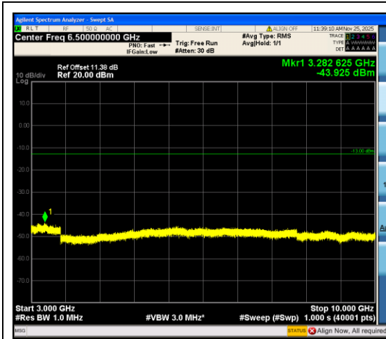
Band12_1.4MHz_QPSK_23017_1RB#0_3000~10000_3000~10000
