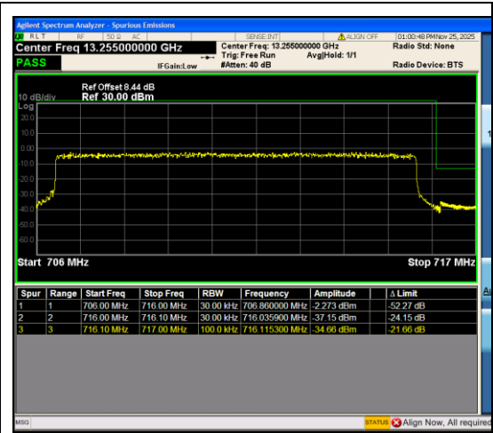
Band12_10MHz_QPSK_23130_50RB#0
