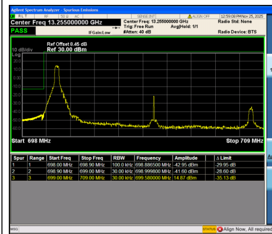
Band12_10MHz_QPSK_23060_1RB#0
