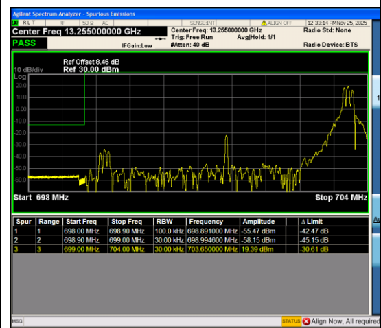
Band12_5MHz_QPSK_23035_1RB#24
