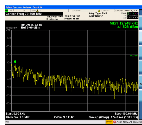
Band12_1.4MHz_QPSK_23017_6RB#0_0.009~0.15_0.009~0.15
