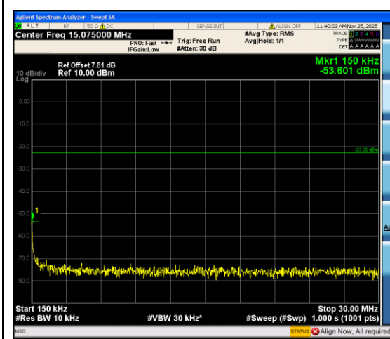
Band12_1.4MHz_QPSK_23017_1RB#5_0.15~30_0.15~30
