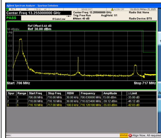
Band12_10MHz_16QAM_23130_1RB#0
