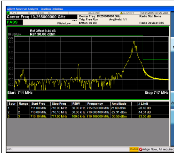
Band12_5MHz_16QAM_23155_1RB#24
