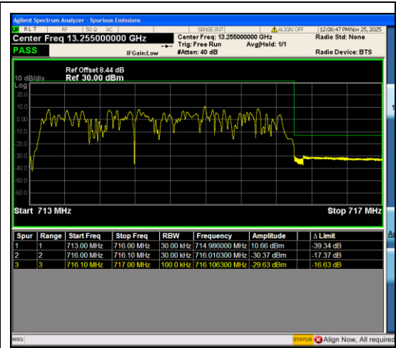
Band12_3MHz_16QAM_23165_15RB#0
