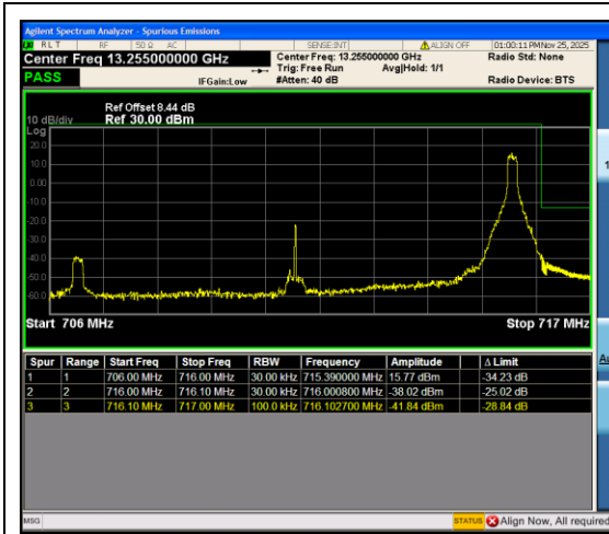
Band12_10MHz_QPSK_23130_1RB#49
