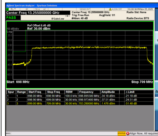
Band12_10MHz_QPSK_23060_50RB#0
