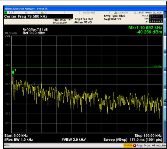
Band12_1.4MHz_QPSK_23017_1RB#5_0.009~0.15_0.009~0.15
