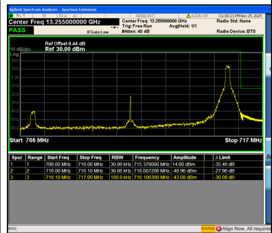
Band12_10MHz_16QAM_23130_1RB#49
