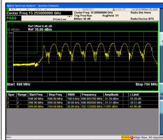
Band12_5MHz_QPSK_23035_25RB#0
