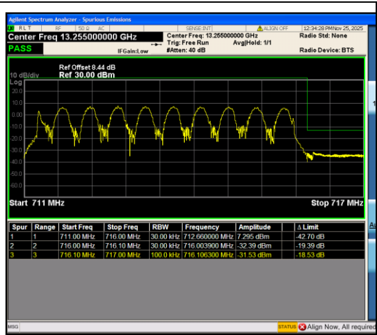
Band12_5MHz_QPSK_23155_25RB#0
