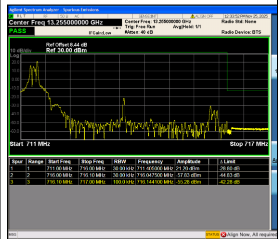
Band12_5MHz_QPSK_23155_1RB#0
