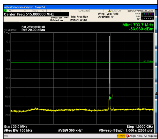
Band12_1.4MHz_QPSK_23017_1RB#5_30~1000_30~1000
