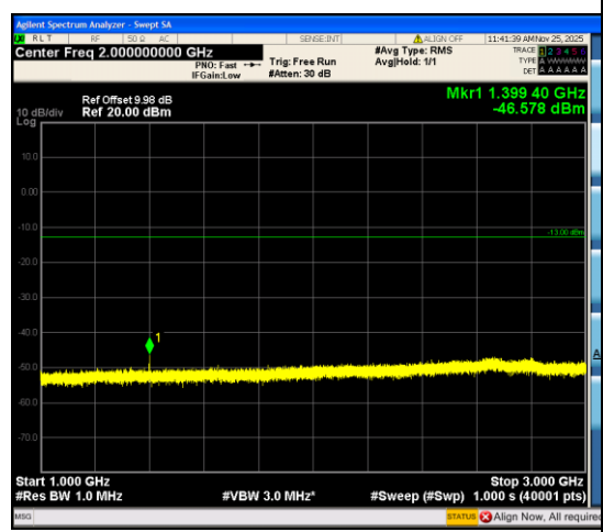
Band12_1.4MHz_QPSK_23017_6RB#0_1000~3000_1000~3000
