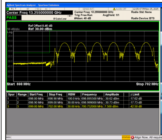
Band12_3MHz_16QAM_23025_15RB#0
