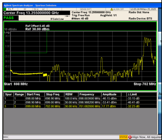
Band12_3MHz_16QAM_23025_1RB#14
