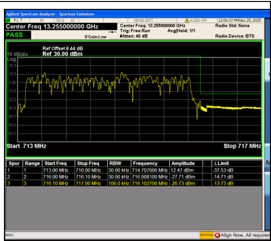
Band12_3MHz_QPSK_23165_15RB#0
