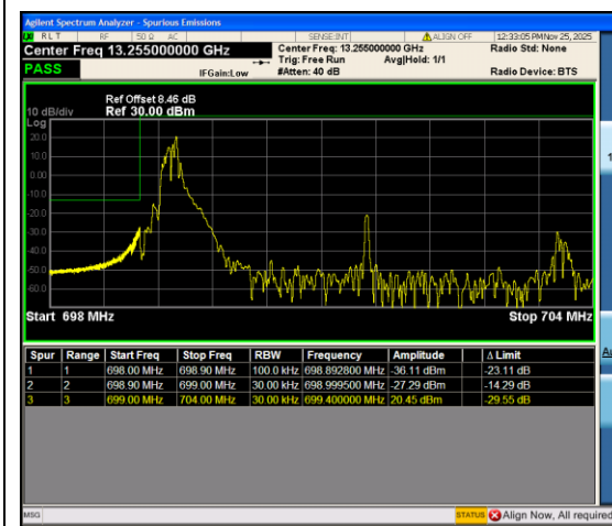
Band12_5MHz_16QAM_23035_1RB#0
