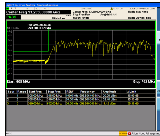
Band12_3MHz_QPSK_23025_15RB#0
