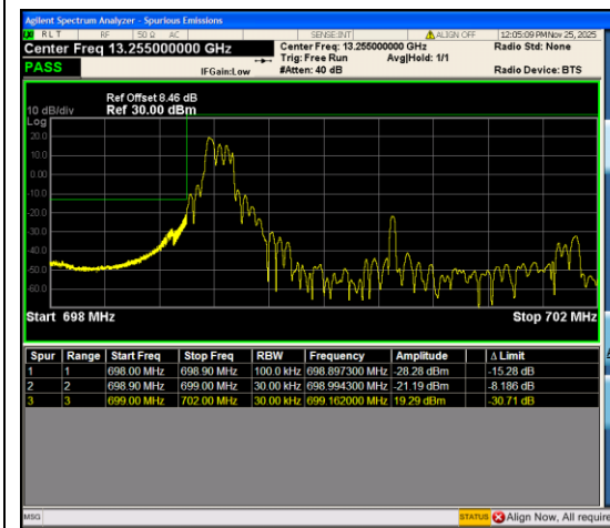
Band12_3MHz_16QAM_23025_1RB#0
