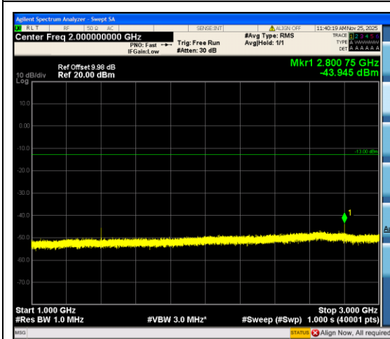
Band12_1.4MHz_QPSK_23017_1RB#5_1000~3000_1000~3000
