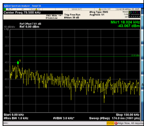
Band12_1.4MHz_QPSK_23095_1RB#0_0.009~0.15_0.009~0.15
