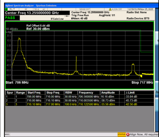
Band12_10MHz_QPSK_23130_1RB#0
