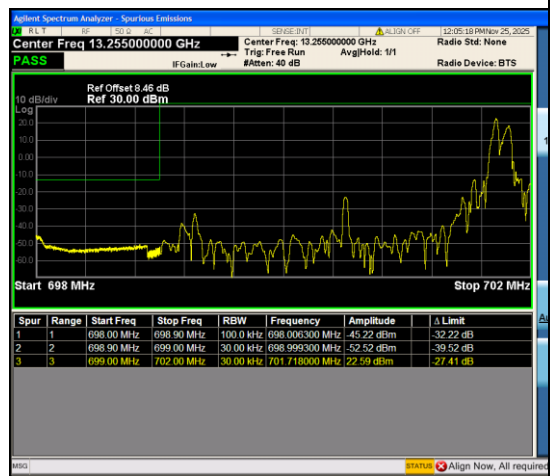
Band12_3MHz_QPSK_23025_1RB#14
