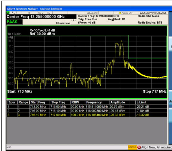
Band12_3MHz_16QAM_23165_1RB#14
