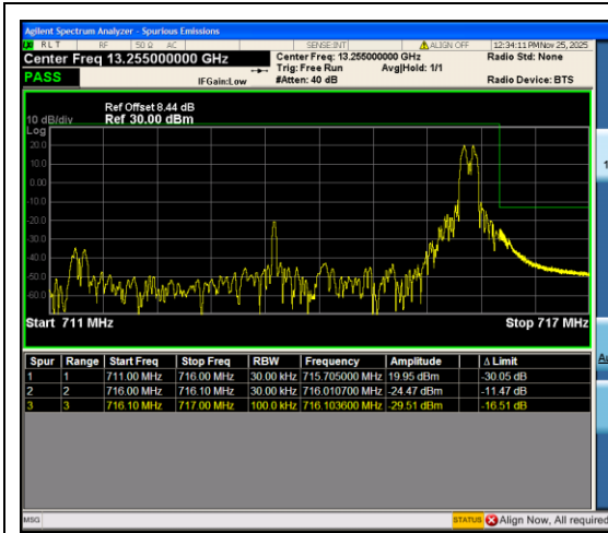
Band12_5MHz_QPSK_23155_1RB#24
