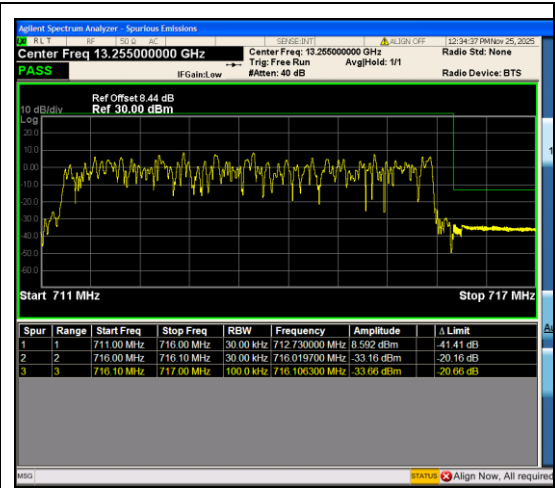
Band12_5MHz_16QAM_23155_25RB#0
