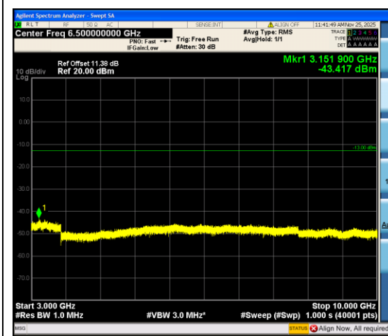
Band12_1.4MHz_QPSK_23017_6RB#0_3000~10000_3000~10000
