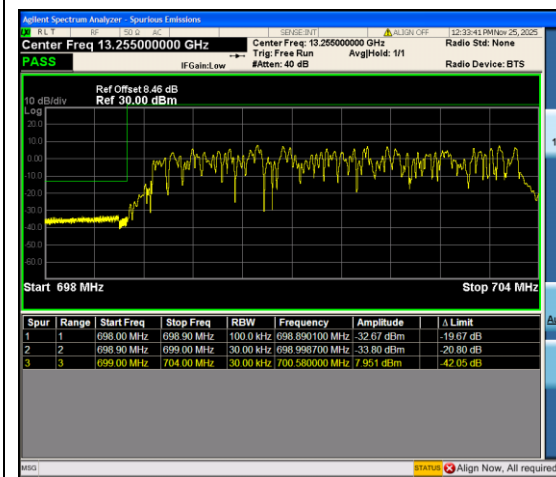
Band12_5MHz_16QAM_23035_25RB#0
