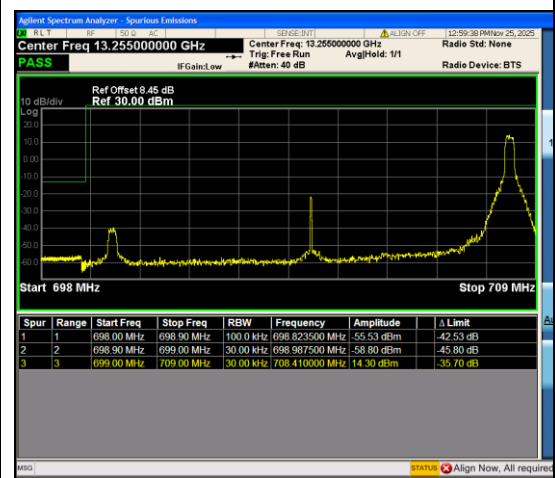
Band12_10MHz_16QAM_23060_1RB#49
