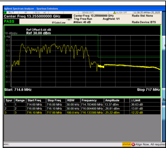
Band12_1.4MHz_16QAM_23173_6RB#0
