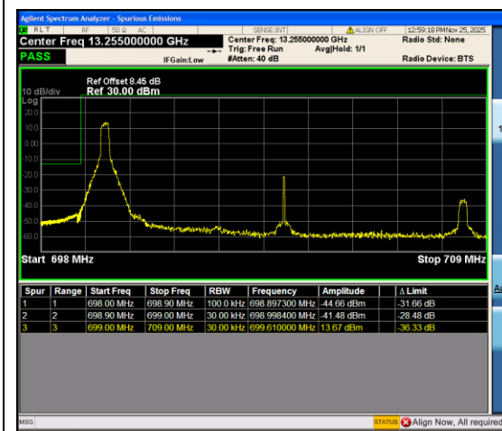
Band12_10MHz_16QAM_23060_1RB#0
