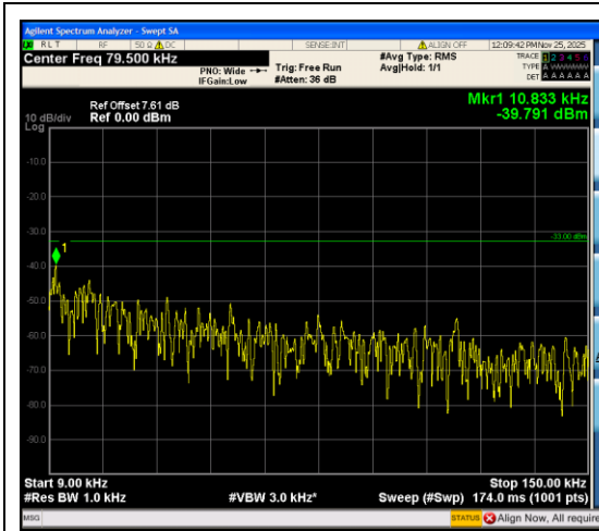
Band12_3MHz_QPSK_23025_15RB#0_0.009~0.15_0.009~0.15
