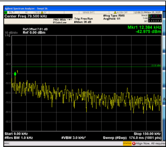
Band12_3MHz_QPSK_23025_1RB#14_0.009~0.15_0.009~0.15
