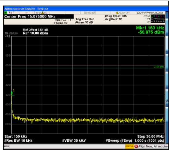
Band12_3MHz_QPSK_23025_15RB#0_0.15~30_0.15~30
