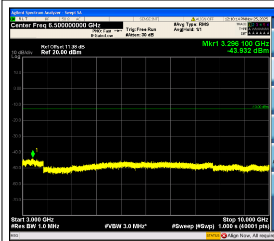
Band12_3MHz_QPSK_23025_15RB#0_3000~10000_3000~10000
