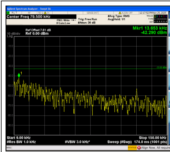
Band12_3MHz_QPSK_23165_15RB#0_0.009~0.15_0.009~0.15
