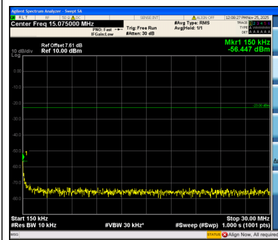
Band12_3MHz_QPSK_23025_1RB#14_0.15~30_0.15~30
