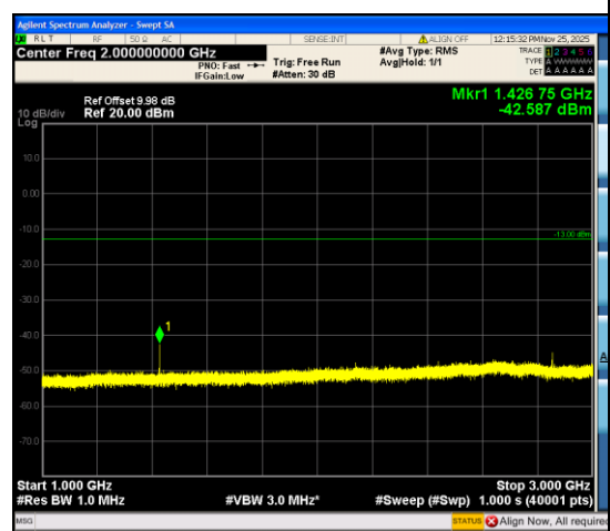
Band12_3MHz_QPSK_23165_1RB#0_1000~3000
