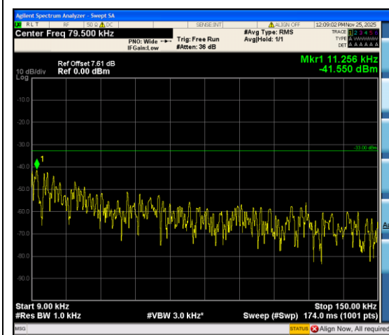
Band12_3MHz_16QAM_23025_1RB#14_0.009~ 0.15_0.009~0.15
