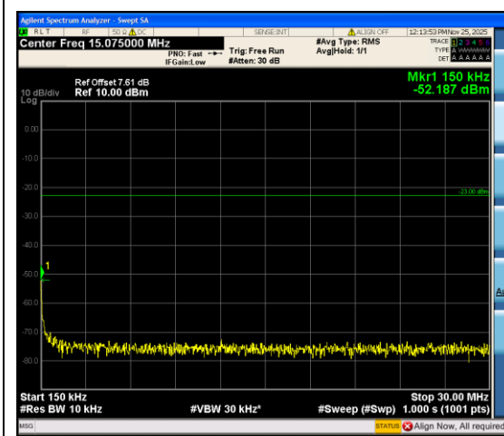
Band12_3MHz_QPSK_23095_15RB#0_0.15~30_0.15~30
