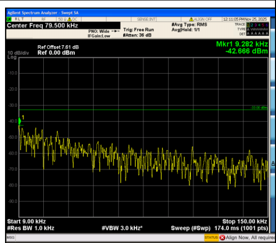
Band12_3MHz_QPSK_23095_1RB#0_0.009~0.15_0.009~0.15
