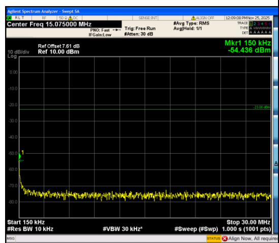
Band12_3MHz_16QAM_23025_1RB#14_0.15~3 0_0.15~30
