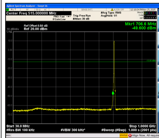
Band12_3MHz_QPSK_23165_15RB#0_30~1000_30~1000
