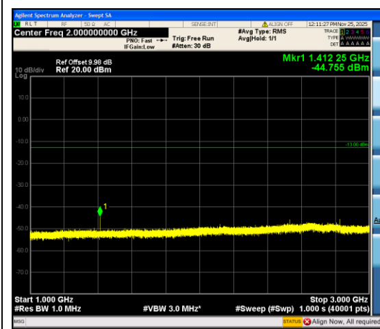
Band12_3MHz_QPSK_23095_1RB#0_1000~3000_0_1000~3000
