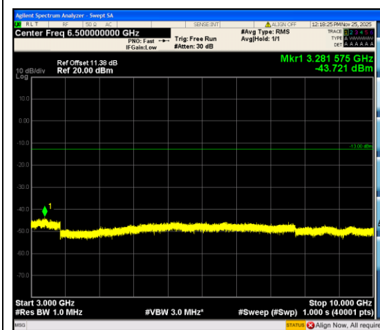
Band12_3MHz_QPSK_23165_15RB#0_3000~10000_3000~10000
