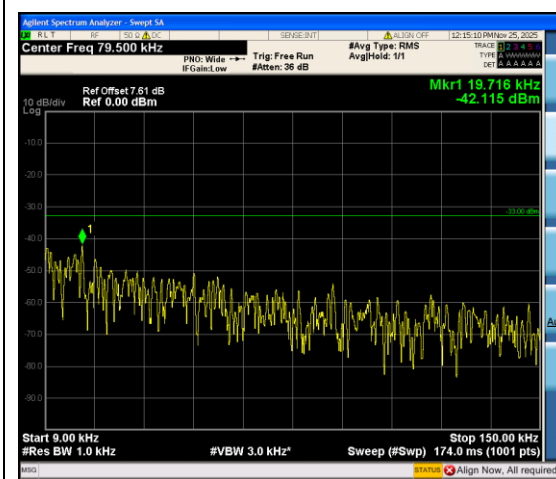
Band12_3MHz_QPSK_23165_1RB#0_0.009~0.15
