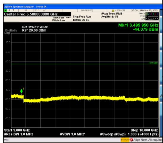
Band12_3MHz_16QAM_23025_1RB#0_3000~1 0000_3000~10000
