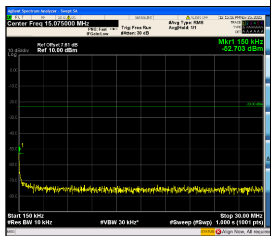
Band12_3MHz_QPSK_23165_1RB#0_0.15~30
