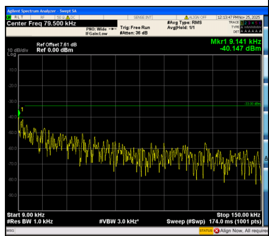
Band12_3MHz_QPSK_23095_15RB#0_0.009~0.15_0.009~0.15
