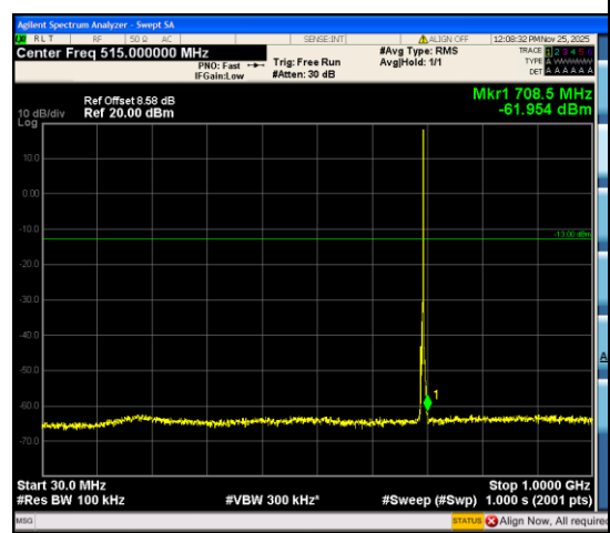
Band12_3MHz_QPSK_23025_1RB#14_30~1000_30~1000
