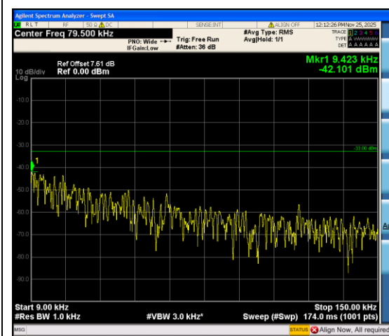
Band12_3MHz_QPSK_23095_1RB#14_0.009~0.15_0.009~0.15
