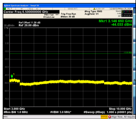
Band12_3MHz_QPSK_23025_1RB#14_3000~10000_3000~10000
