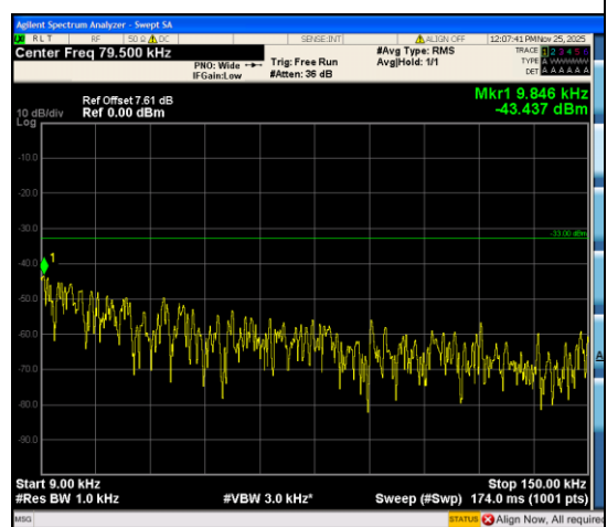
Band12_3MHz_16QAM_23025_1RB#0_0.009~0.15_0.009~0.15
