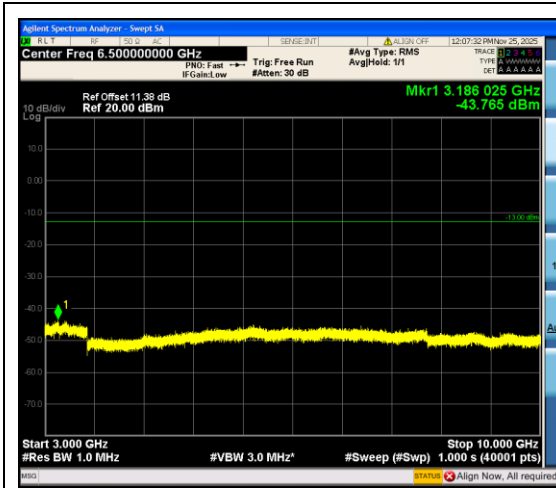
Band12_3MHz_QPSK_23025_1RB#0_3000~10000_3000~10000
