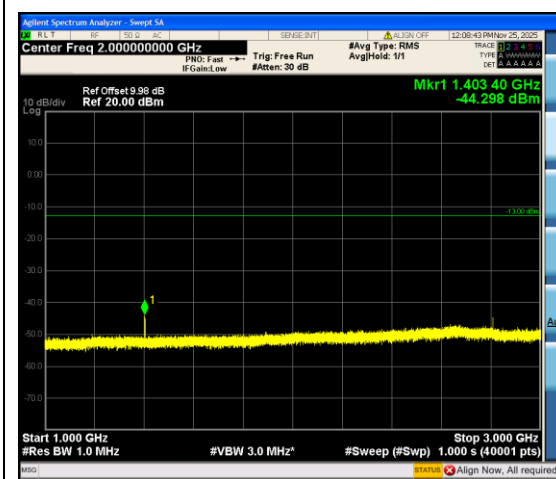
Band12_3MHz_QPSK_23025_1RB#14_1000~3000_1000~3000
