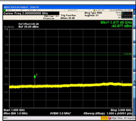
Band12_3MHz_QPSK_23095_1RB#14_1000~3000_1000~3000
