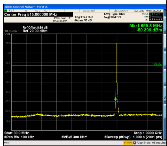
Band12_3MHz_QPSK_23095_15RB#0_30~1000_30~1000
