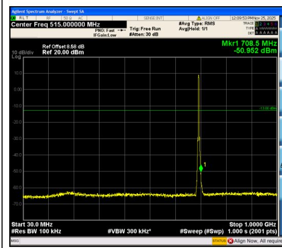
Band12_3MHz_QPSK_23025_15RB#0_30~1000_30~1000
