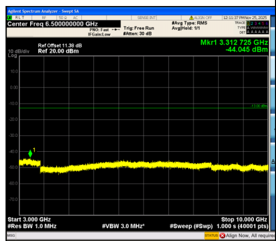
Band12_3MHz_QPSK_23095_1RB#0_3000~10000_000_3000~10000
