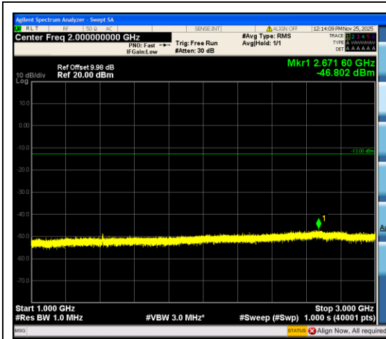
Band12_3MHz_QPSK_23095_15RB#0_1000~3000
