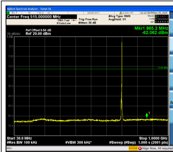
Band12_3MHz_QPSK_23095_1RB#14_30~1000_30~1000
