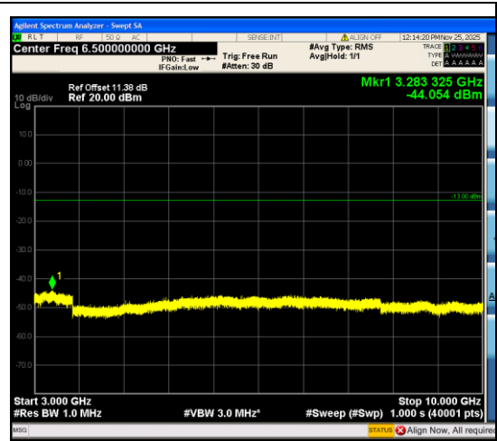
Band12_3MHz_QPSK_23095_15RB#0_3000~10000
