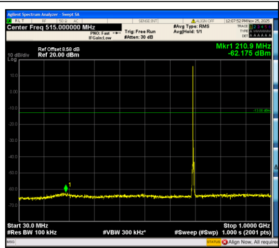
Band12_3MHz_16QAM_23025_1RB#0_30~100 0_30~1000
