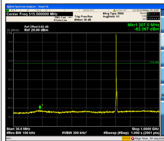
Band12_3MHz_QPSK_23165_1RB#0_30~1000
