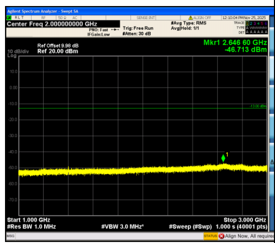
Band12_3MHz_QPSK_23025_15RB#0_1000~3000_1000~3000
