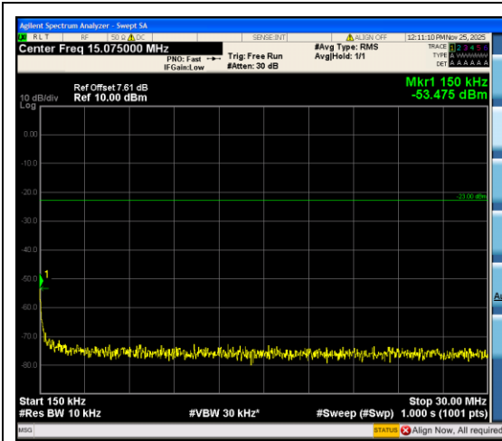
Band12_3MHz_QPSK_23095_1RB#0_0.15~30_0.15~30
