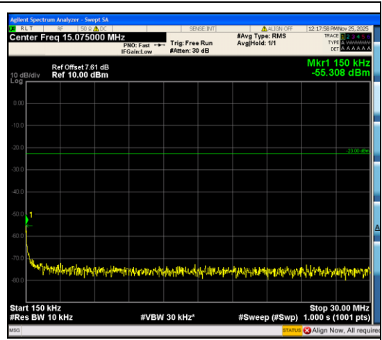
Band12_3MHz_QPSK_23165_15RB#0_0.15~30_0.15~30
