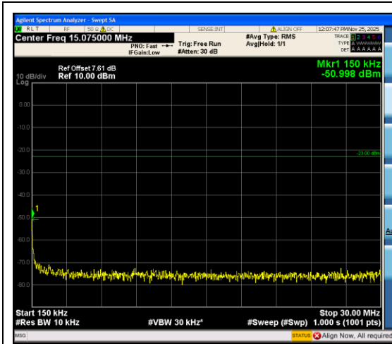
Band12_3MHz_16QAM_23025_1RB#0_0.15~30 _0.15~30
