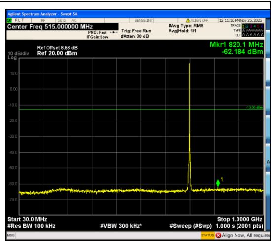
Band12_3MHz_QPSK_23095_1RB#0_30~1000_30~1000
