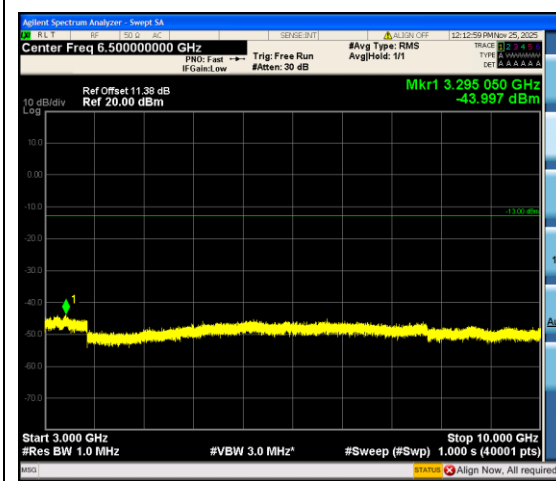
Band12_3MHz_QPSK_23095_1RB#14_3000~10000_3000~10000
