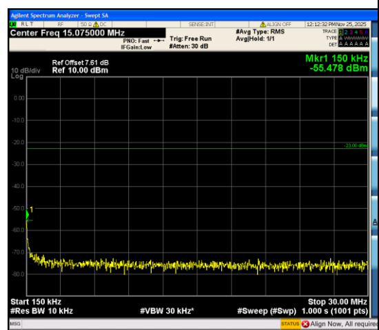
Band12_3MHz_QPSK_23095_1RB#14_0.15~30_0.15~30
