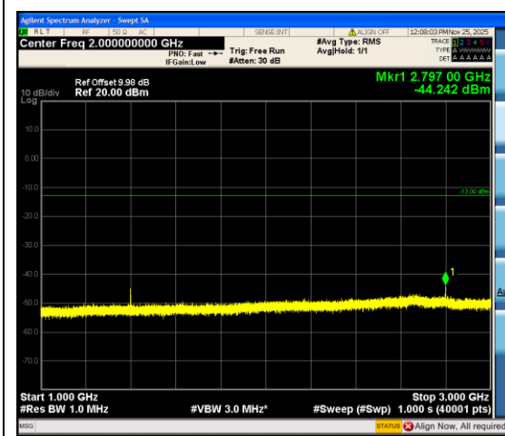
Band12_3MHz_16QAM_23025_1RB#0_1000~3 000_1000~3000
