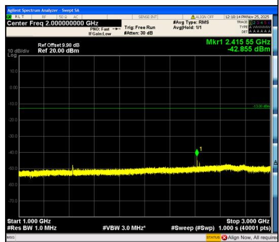
Band12_3MHz_QPSK_23165_15RB#0_1000~3000_1000~3000
