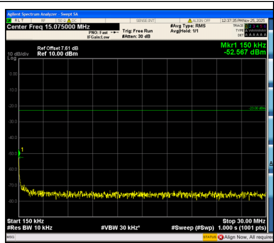
Band12_5MHz_QPSK_23035_25RB#0_0.15~30_0.15~30
