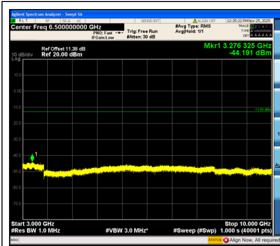
Band12_5MHz_QPSK_23035_1RB#0_3000~10000
