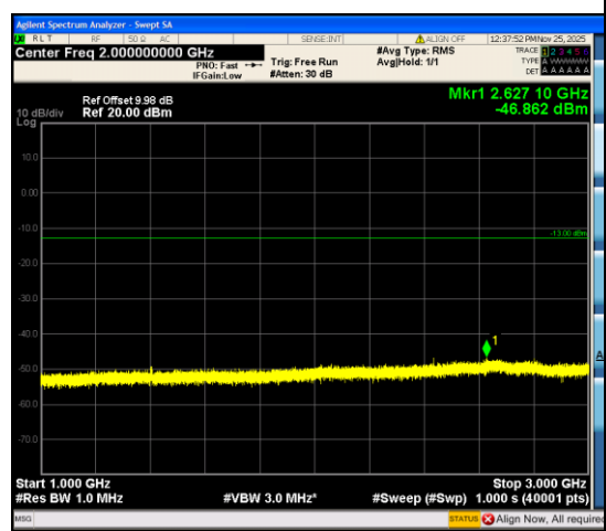
Band12_5MHz_QPSK_23035_25RB#0_1000~3000_1000~3000
