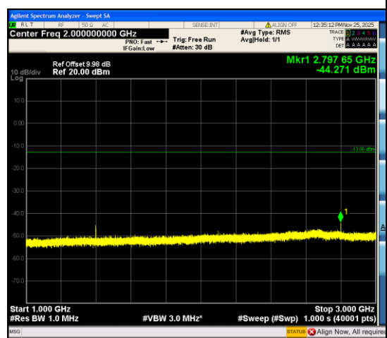
Band12_5MHz_QPSK_23035_1RB#0_1000~30 00_1000~3000
