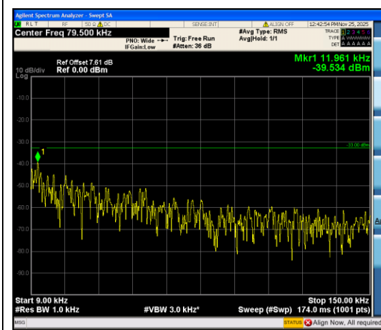
Band12_5MHz_QPSK_23155_1RB#0_0.009~0.15
