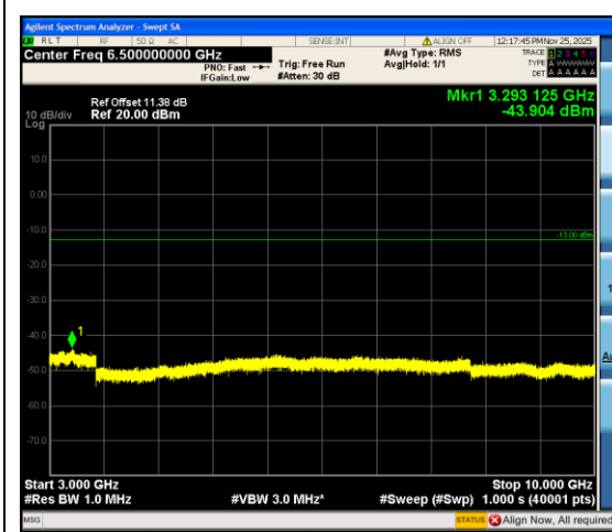
Band12_3MHz_16QAM_23165_1RB#14_3000~10000_3000~10000
