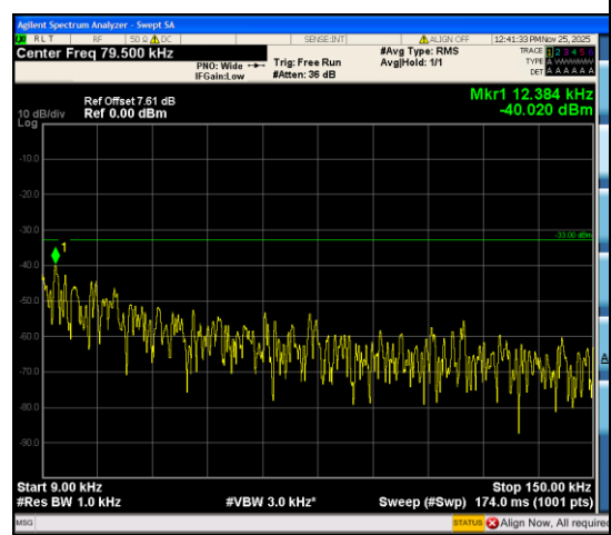
Band12_5MHz_QPSK_23095_25RB#0_0.009~0.15_0.009~0.15
