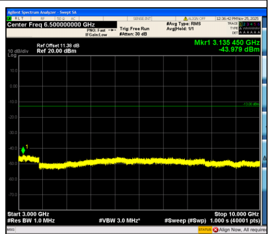
Band12_5MHz_QPSK_23035_1RB#24_3000~10000
