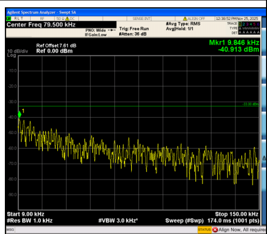
Band12_5MHz_QPSK_23095_1RB#0_0.009~0.15_15_0.009~0.15
