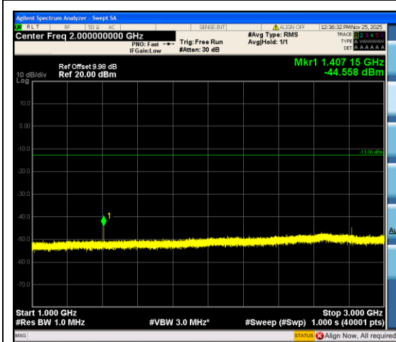
Band12_5MHz_QPSK_23035_1RB#24_1000~3000
