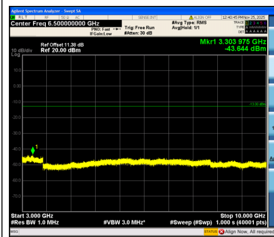
Band12_5MHz_QPSK_23095_1RB#24_3000~10000_000_3000~10000
