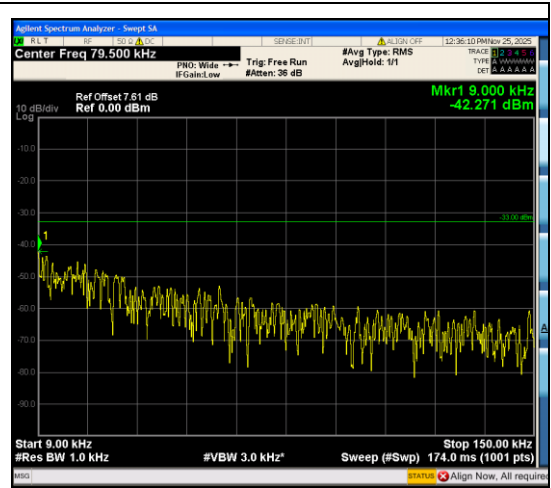
Band12_5MHz_QPSK_23035_1RB#24_0.009~0.15
