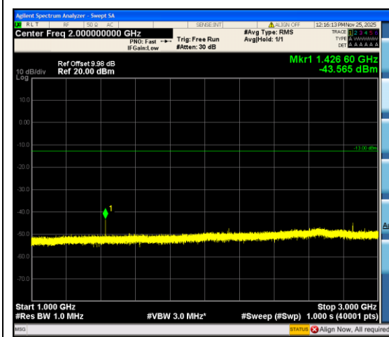
Band12_3MHz_16QAM_23165_1RB#0_1000~3 000_1000~3000
