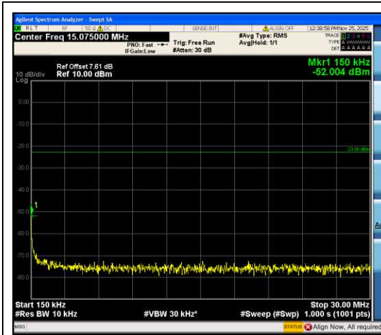
Band12_5MHz_QPSK_23095_1RB#0_0.15~30_0.15~30
