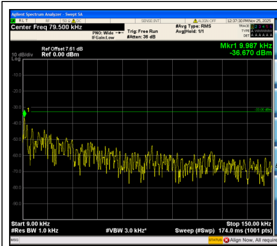
Band12_5MHz_QPSK_23035_25RB#0_0.009~0.15_0.009~0.15
