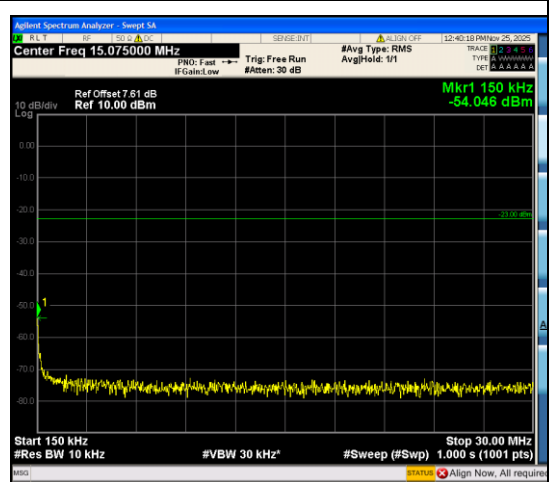
Band12_5MHz_QPSK_23095_1RB#24_0.15~30_0.15~30
