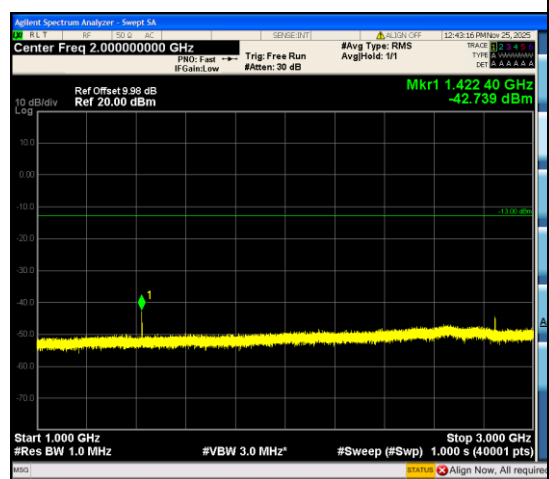
Band12_5MHz_QPSK_23155_1RB#0_1000~3000
