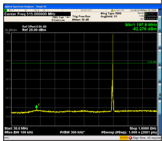
Band12_5MHz_QPSK_23035_1RB#24_30~1000
