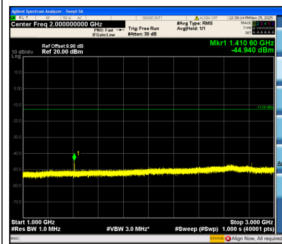
Band12_5MHz_QPSK_23095_1RB#0_1000~3000_0_1000~3000
