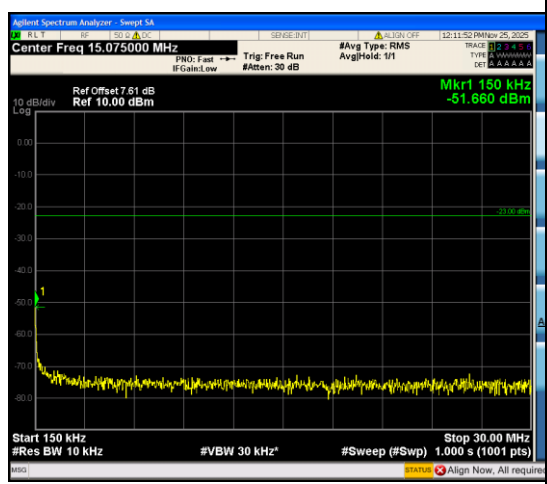
Band12_3MHz_16QAM_23095_1RB#0_0.15~30 _0.15~30
