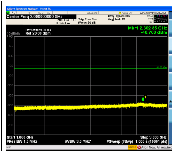
Band12_5MHz_QPSK_23095_25RB#0_1000~3000
