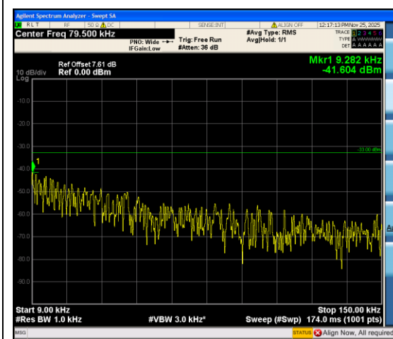
Band12_3MHz_16QAM_23165_1RB#14_0.009~ 0.15_0.009~0.15
