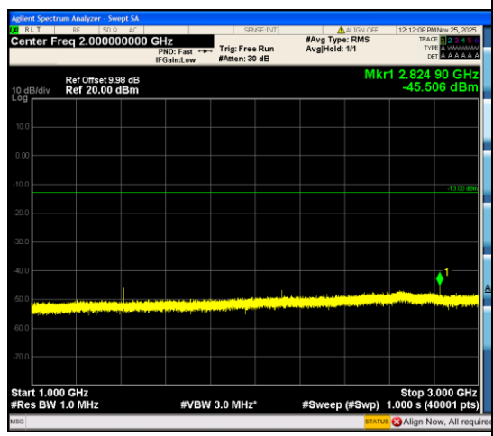
Band12_3MHz_16QAM_23095_1RB#0_1000~3 000_1000~3000
