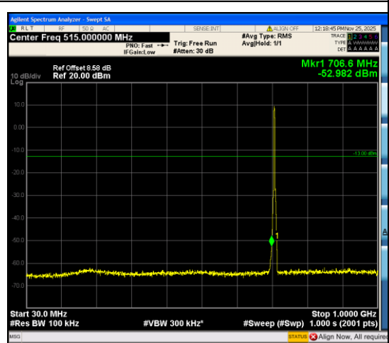
Band12_3MHz_16QAM_23165_15RB#0_30~1000_30~1000
