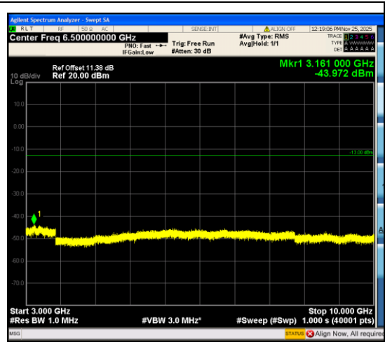
Band12_3MHz_16QAM_23165_15RB#0_3000~ 10000_3000~10000
