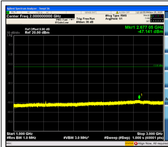
Band12_3MHz_16QAM_23165_15RB#0_1000~ 3000_1000~3000
