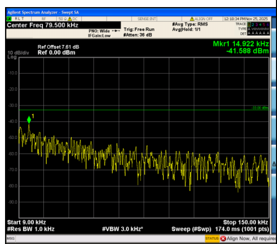
Band12_3MHz_16QAM_23165_15RB#0_0.009~0.15_0.009~0.15
