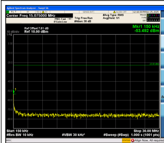
Band12_3MHz_16QAM_23165_15RB#0_0.15~30_0.15~30
