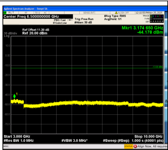
Band12_3MHz_16QAM_23025_15RB#0_3000~ 10000_3000~10000
