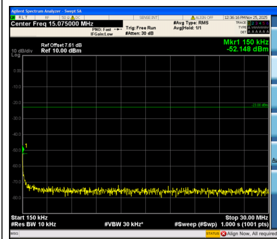
Band12_5MHz_QPSK_23035_1RB#24_0.15~30
