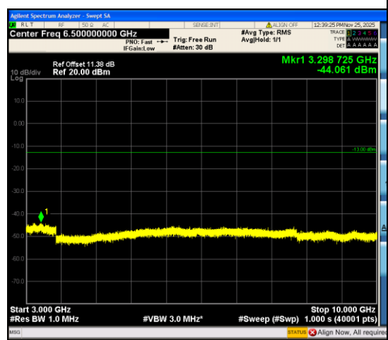
Band12_5MHz_QPSK_23095_1RB#0_3000~10000_000_3000~10000
