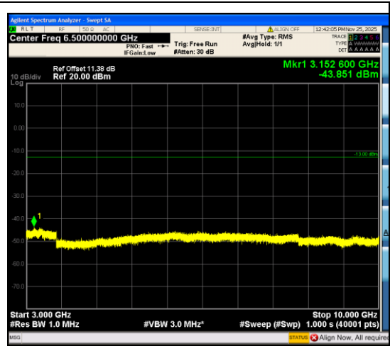
Band12_5MHz_QPSK_23095_25RB#0_3000~10000
