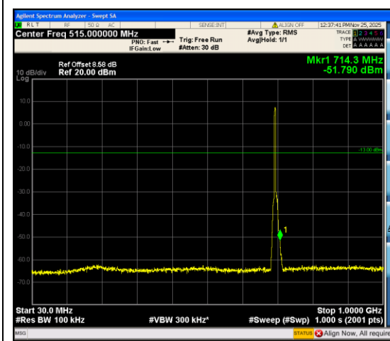
Band12_5MHz_QPSK_23035_25RB#0_30~1000_30~1000
