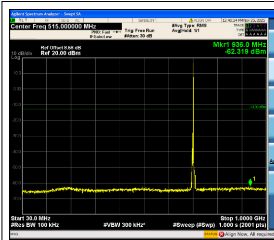
Band12_5MHz_QPSK_23095_1RB#24_30~1000_30~1000
