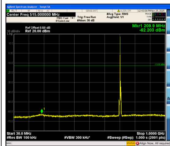
Band12_5MHz_QPSK_23155_1RB#0_30~1000
