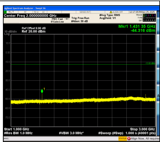
Band12_3MHz_16QAM_23165_1RB#14_1000~3000_1000~3000
