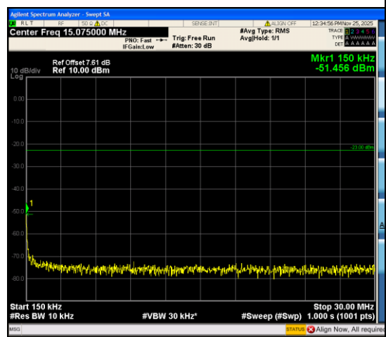
Band12_5MHz_QPSK_23035_1RB#0_0.15~30_ 0.15~30
