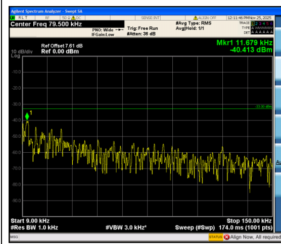
Band12_3MHz_16QAM_23095_1RB#0_0.009~0 .15_0.009~0.15
