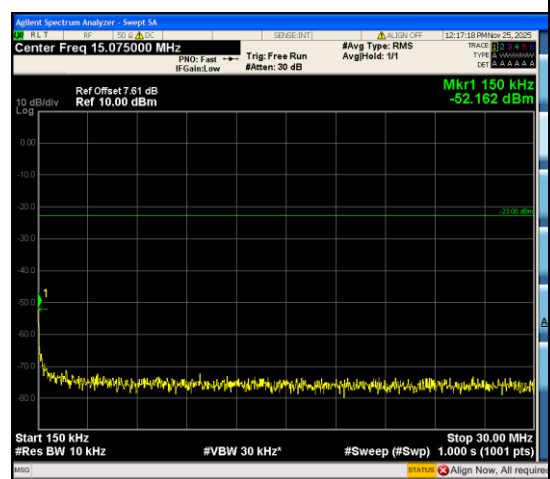
Band12_3MHz_16QAM_23165_1RB#14_0.15~3 0_0.15~30
