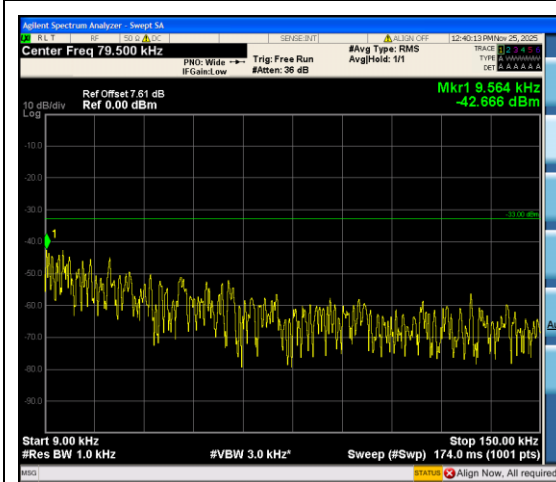
Band12_5MHz_QPSK_23095_1RB#24_0.009~0.15_0.009~0.15
