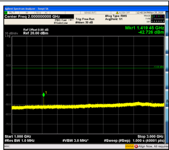
Band12_5MHz_QPSK_23095_1RB#24_1000~3000_000_1000~3000
