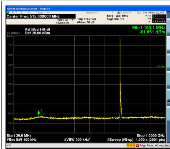
Band12_3MHz_16QAM_23165_1RB#14_30~1000_30~1000
