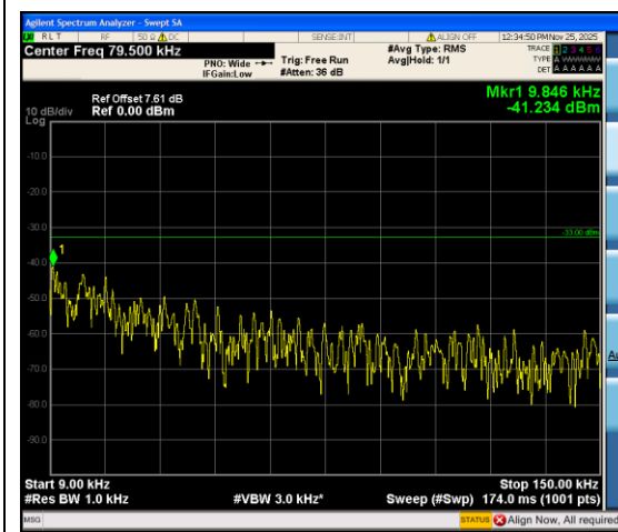
Band12_5MHz_QPSK_23035_1RB#0_0.009~0.1 5_0.009~0.15
