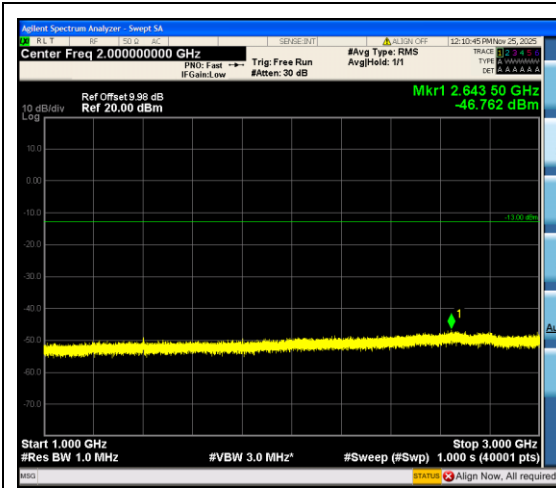
Band12_3MHz_16QAM_23025_15RB#0_1000~ 3000_1000~3000
