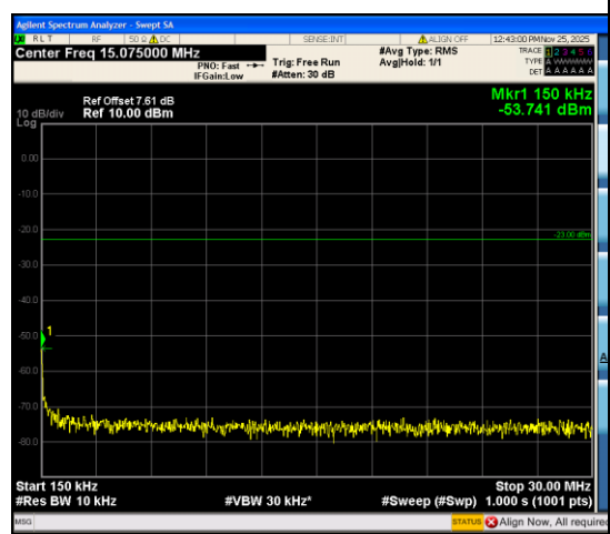
Band12_5MHz_QPSK_23155_1RB#0_0.15~30
