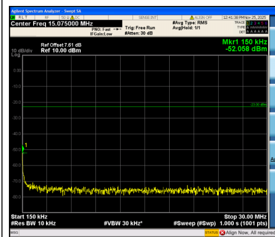
Band12_5MHz_QPSK_23095_25RB#0_0.15~30_0.15~30
