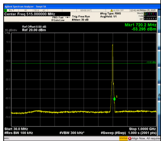
Band12_5MHz_QPSK_23095_25RB#0_30~1000_0_30~1000
