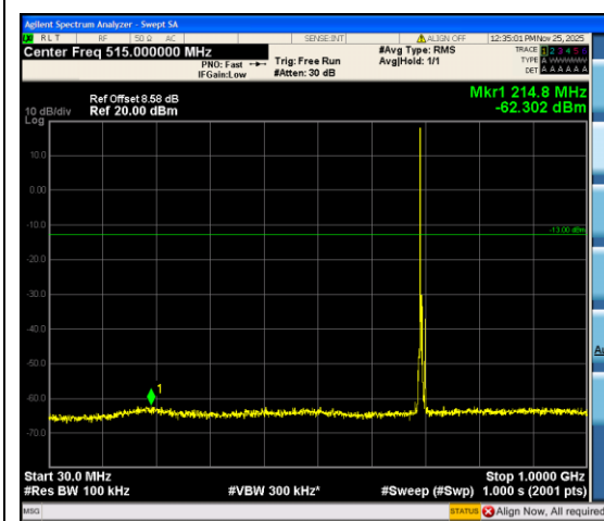
Band12_5MHz_QPSK_23035_1RB#0_30~1000_ 30~1000
