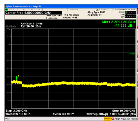
Band12_5MHz_QPSK_23035_25RB#0_3000~10000_3000~10000
