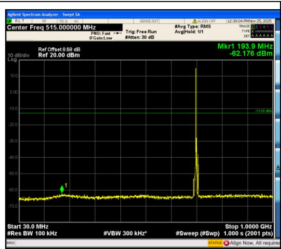
Band12_5MHz_QPSK_23095_1RB#0_30~1000_30~1000
