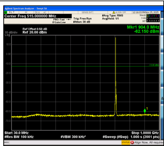
Band12_3MHz_16QAM_23165_1RB#0_30~100 0_30~1000
