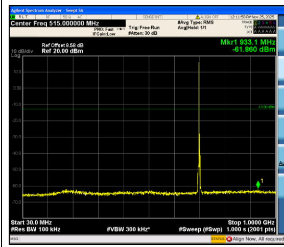
Band12_3MHz_16QAM_23095_1RB#0_30~100 0_30~1000
