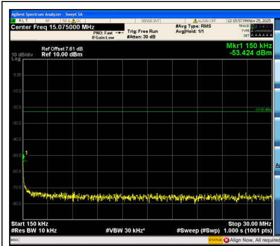
Band12_3MHz_16QAM_23165_1RB#0_0.15~30 _0.15~30
