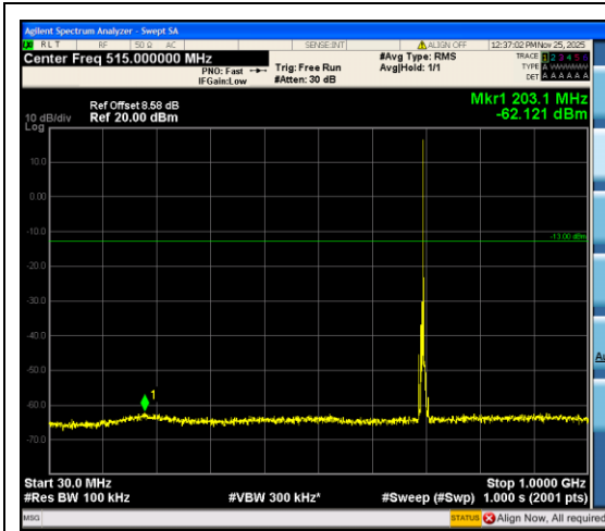
Band12_5MHz_16QAM_23035_1RB#24_30~1000_00_30~1000
