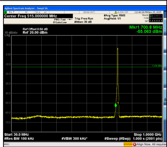
Band12_5MHz_16QAM_23155_25RB#0_30~1000_30~1000
