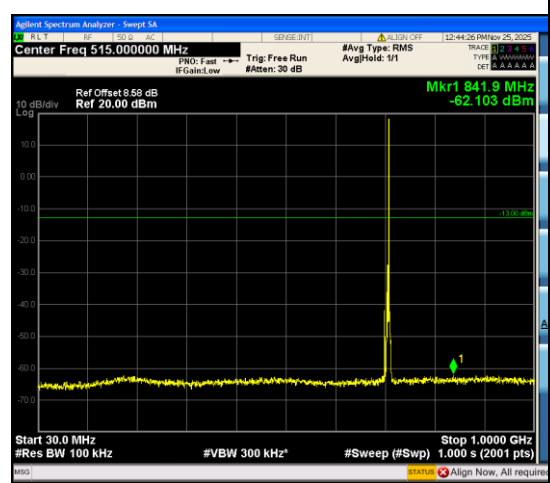
Band12_5MHz_QPSK_23155_1RB#24_30~1000_30~1000
