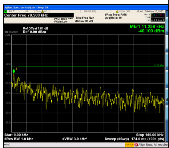
Band12_5MHz_16QAM_23155_25RB#0_0.009~0.15_0.009~0.15
