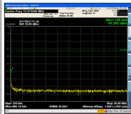
Band12_5MHz_16QAM_23035_25RB#0_0.15~30_0.15~30
