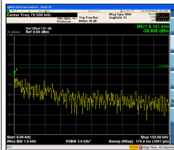
Band12_5MHz_16QAM_23155_1RB#24_0.009~ 0.15_0.009~0.15
