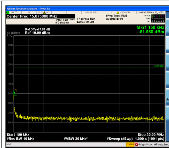
Band12_5MHz_16QAM_23155_1RB#0_0.15~30 _0.15~30
