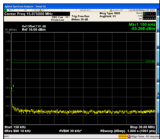
Band12_5MHz_16QAM_23155_1RB#24_0.15~3 0_0.15~30
