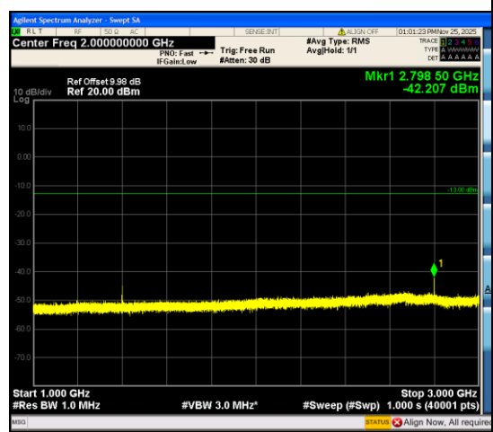
Band12_10MHz_QPSK_23060_1RB#0_1000~3 000_1000~3000
