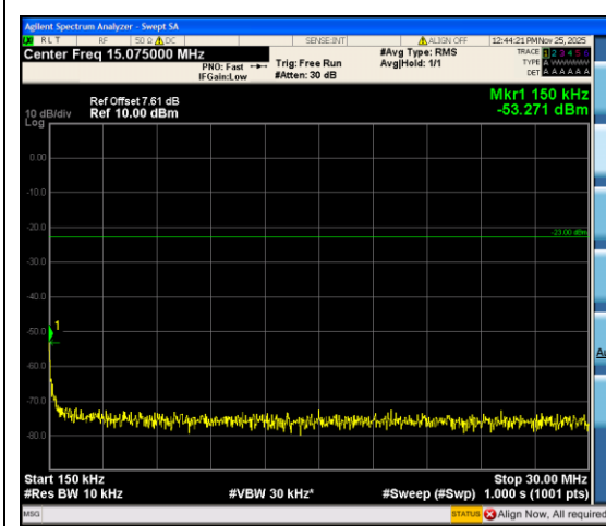
Band12_5MHz_QPSK_23155_1RB#24_0.15~30_0.15~30
