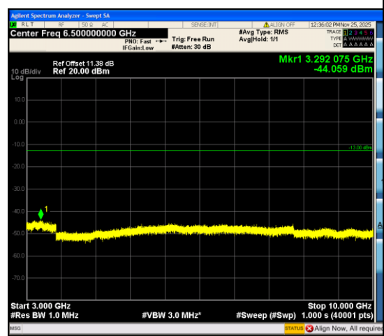
Band12_5MHz_16QAM_23035_1RB#0_3000~1 0000_3000~10000
