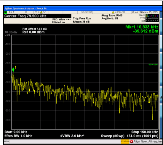
Band12_5MHz_QPSK_23155_1RB#24_0.009~0.15_0.009~0.15
