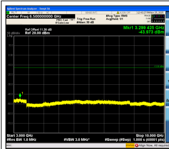
Band12_5MHz_QPSK_23155_1RB#0_3000~1000_3000~10000
