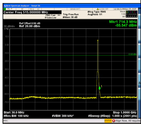
Band12_5MHz_16QAM_23035_25RB#0_30~1000_30~1000
