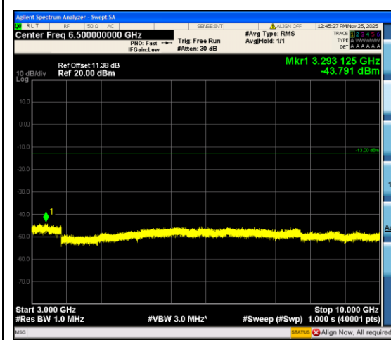
Band12_5MHz_16QAM_23155_1RB#24_3000~10000_3000~10000
