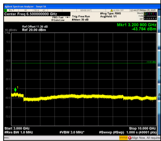
Band12_5MHz_16QAM_23155_1RB#0_3000~1 0000_3000~10000
