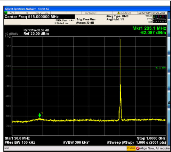
Band12_5MHz_16QAM_23155_1RB#0_30~1000 0_30~1000
