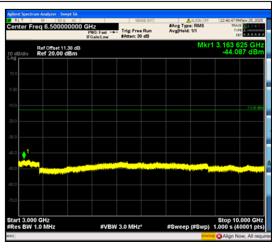
Band12_5MHz_16QAM_23155_25RB#0_3000~ 10000_3000~10000
