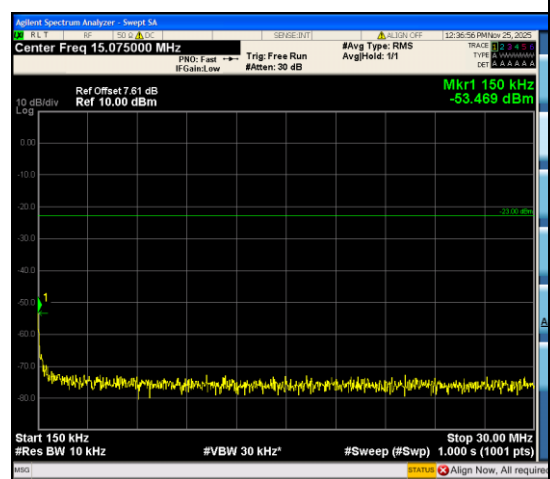
Band12_5MHz_16QAM_23035_1RB#24_0.15~3 0_0.15~30
