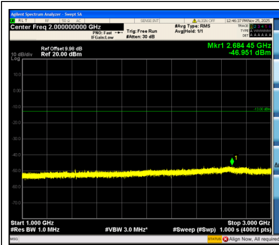
Band12_5MHz_16QAM_23155_25RB#0_1000~ 3000_1000~3000
