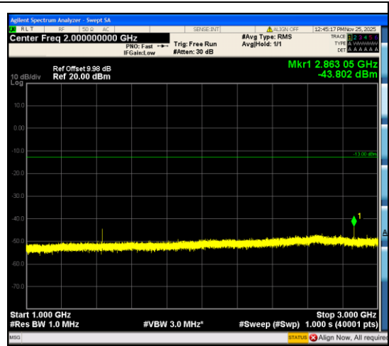
Band12_5MHz_16QAM_23155_1RB#24_1000~3000_1000~3000
