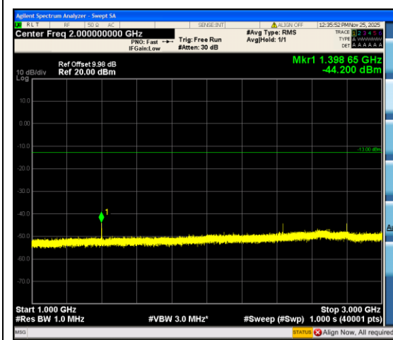
Band12_5MHz_16QAM_23035_1RB#0_1000~3 000_1000~3000
