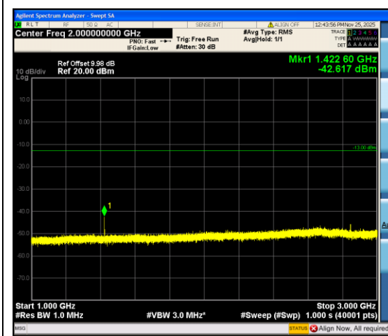
Band12_5MHz_16QAM_23155_1RB#0_1000~3 000_1000~3000
