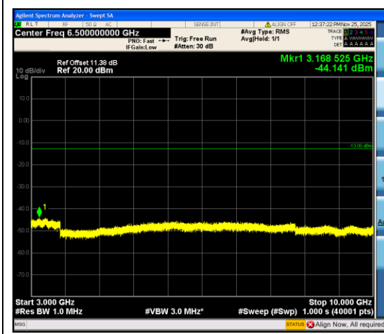
Band12_5MHz_16QAM_23035_1RB#24_3000~10000_3000~10000
