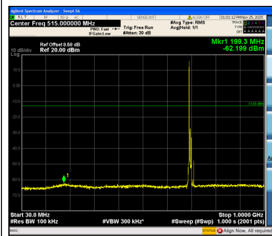
Band12_10MHz_QPSK_23060_1RB#0_30~1000 _30~1000
