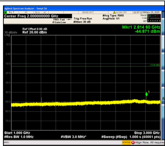
Band12_5MHz_16QAM_23035_1RB#24_1000~3000_1000~3000
