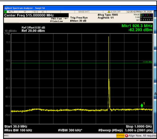
Band12_5MHz_16QAM_23035_1RB#0_30~1000 0_30~1000
