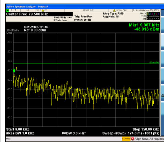
Band12_10MHz_QPSK_23060_1RB#0_0.009~0. 15_0.009~0.15
