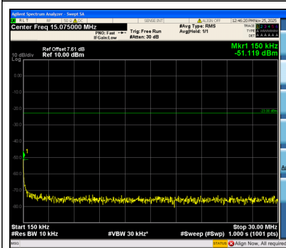
Band12_5MHz_16QAM_23155_25RB#0_0.15~30_0.15~30
