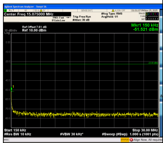
Band12_10MHz_QPSK_23060_1RB#0_0.15~30 _0.15~30
