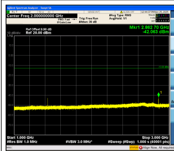
Band12_5MHz_QPSK_23155_1RB#24_1000~3000_1000~3000
