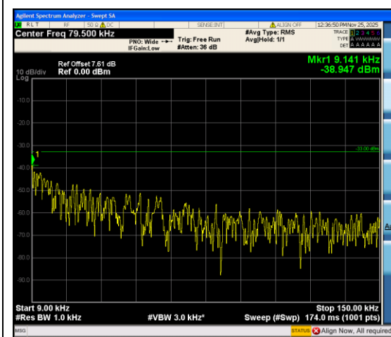
Band12_5MHz_16QAM_23035_1RB#24_0.009~ 0.15_0.009~0.15
