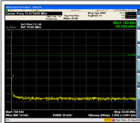
Band12_5MHz_16QAM_23035_1RB#0_0.15~30 _0.15~30
