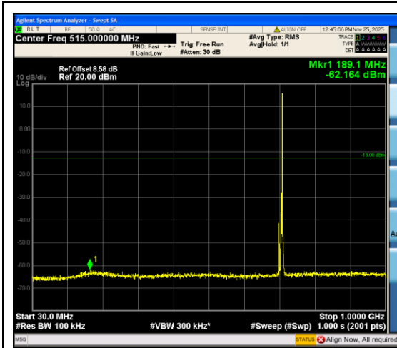
Band12_5MHz_16QAM_23155_1RB#24_30~1000_30~1000
