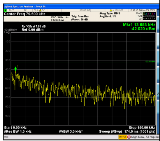
Band12_5MHz_16QAM_23035_25RB#0_0.009~0.15_0.009~0.15
