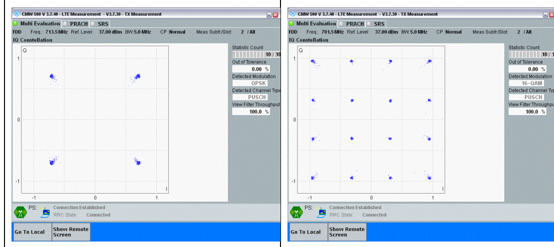
Band12-5MHz-QPSK-23155-25RB#0-PASS
