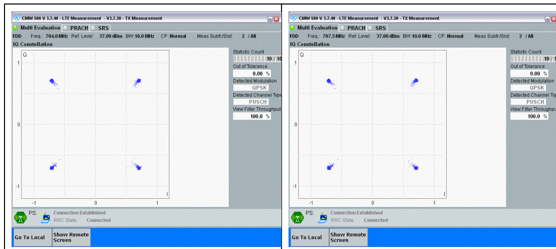
Band12-10MHz-QPSK-23060-50RB#0-PASS
