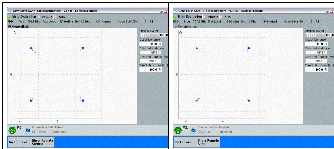
Band12-3MHz-QPSK-23025-15RB#0-PASS
