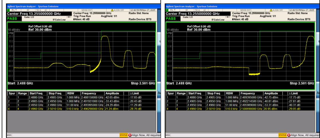
Band41_5MHz_16QAM_39675_1RB#0
