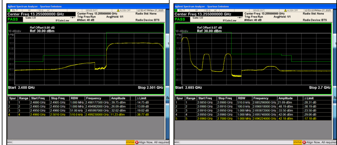
Band41_5MHz_16QAM_39675_25RB#0
